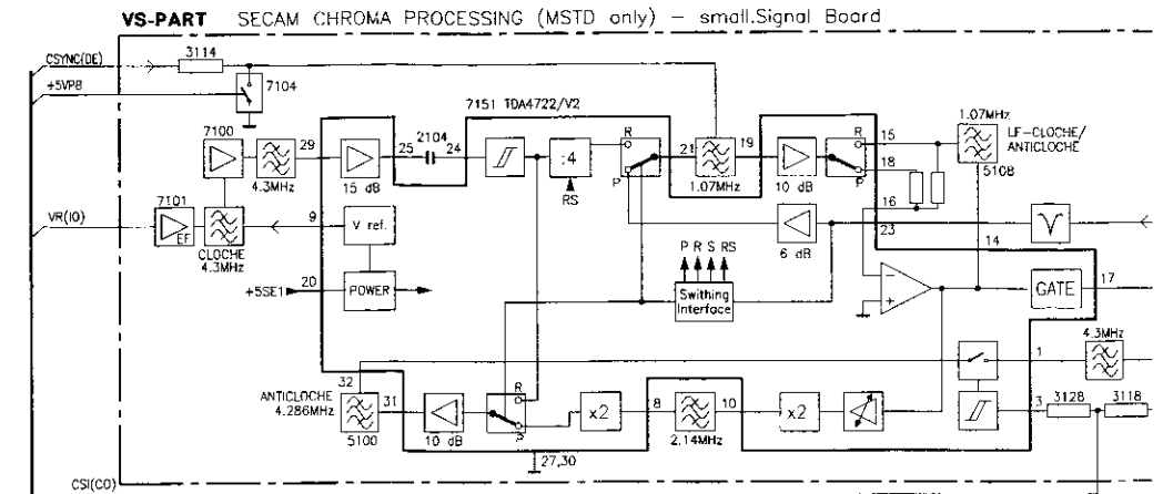
VS-PART SECAM CHROMA PROCESSING (MSTD only) - small.Signal Board
