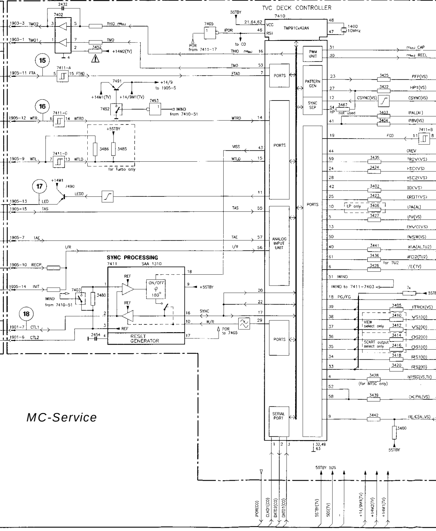
DECK ELECTRONIC (DE) Small Signal Board
