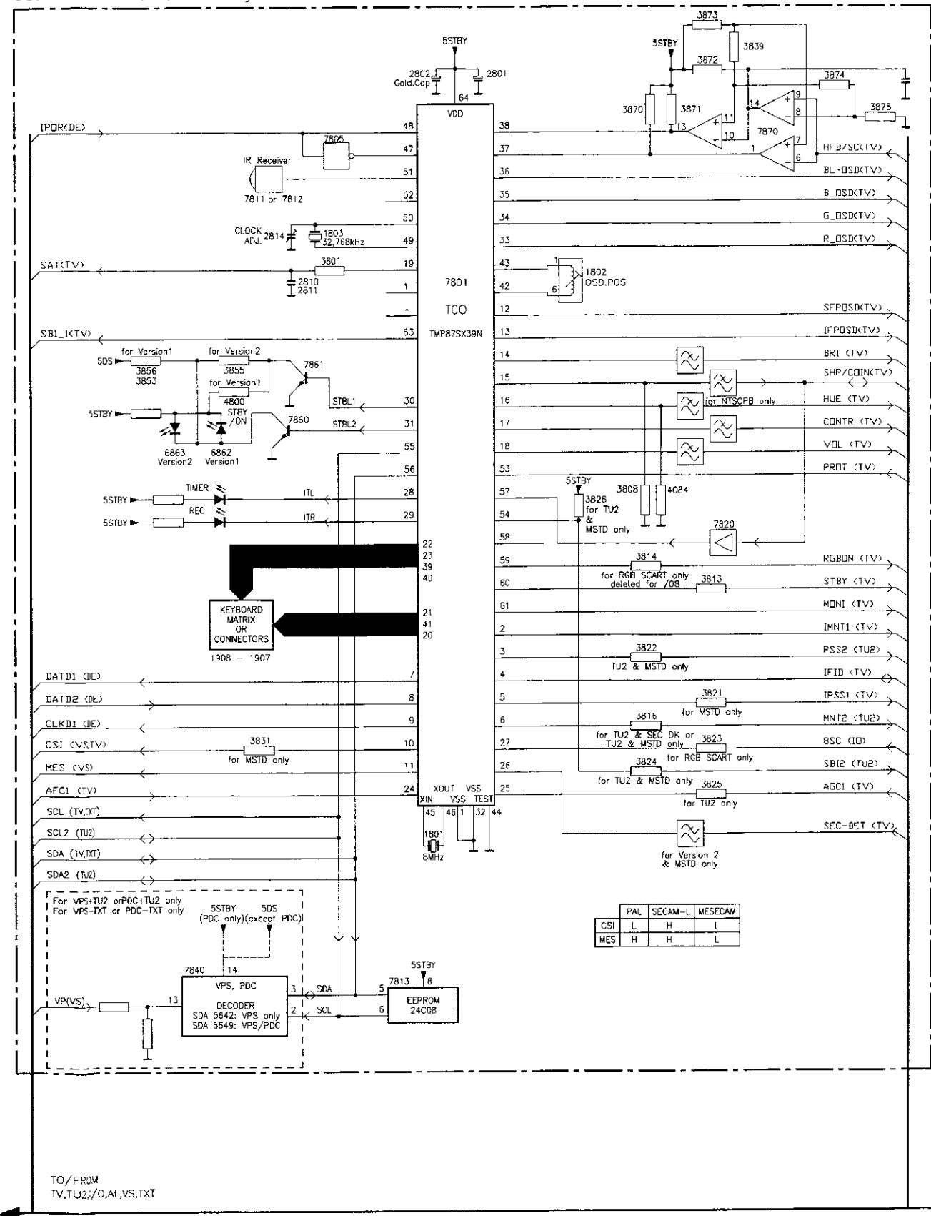
CONTROL PART (CO) Small Signal Board
