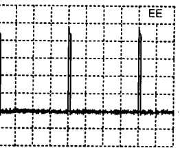
A: DC, 1 V/Div, 5ms/Div Resistor 3569
