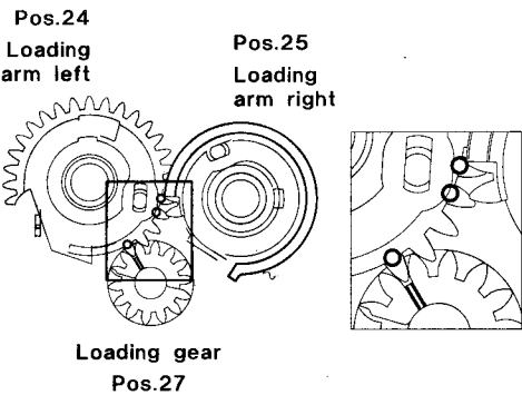
Top view 1
