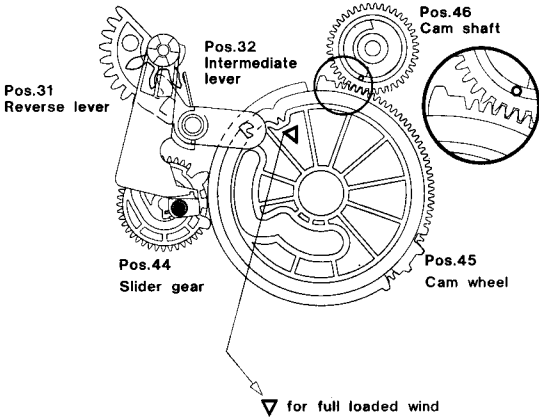
Top view 2
