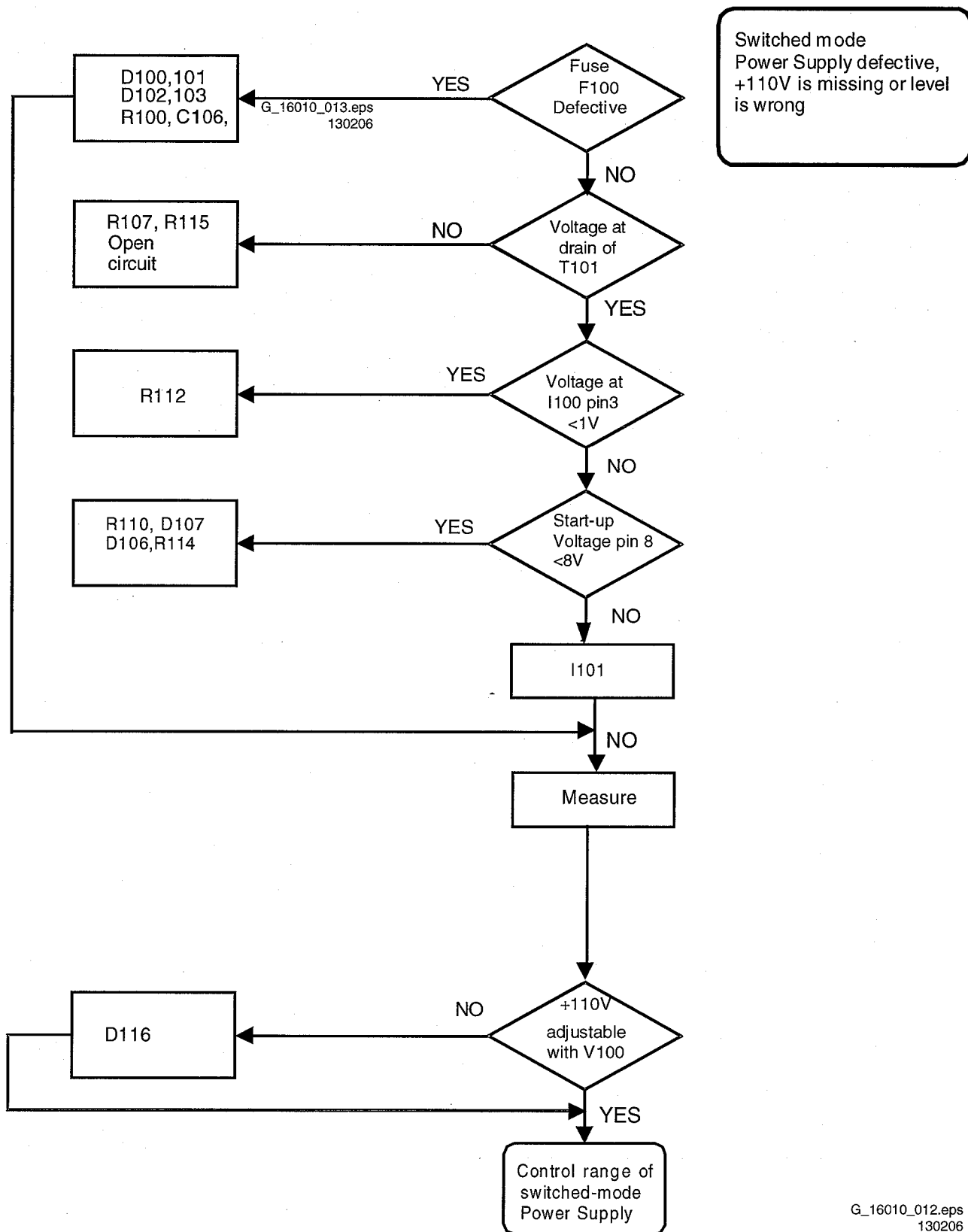
Figure 5-2 Fault Tracing
