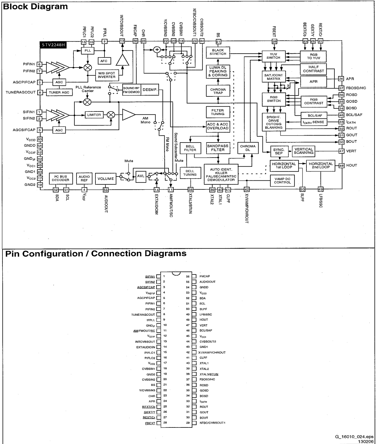
Figure 9-3 Internal block diagram and pin configuration
