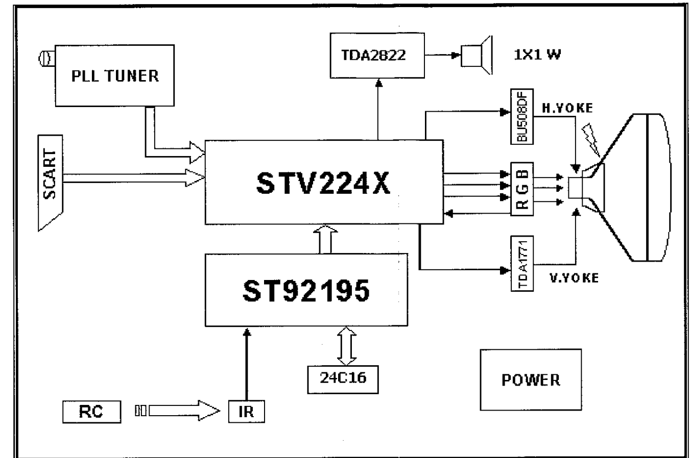
Block Diagram
