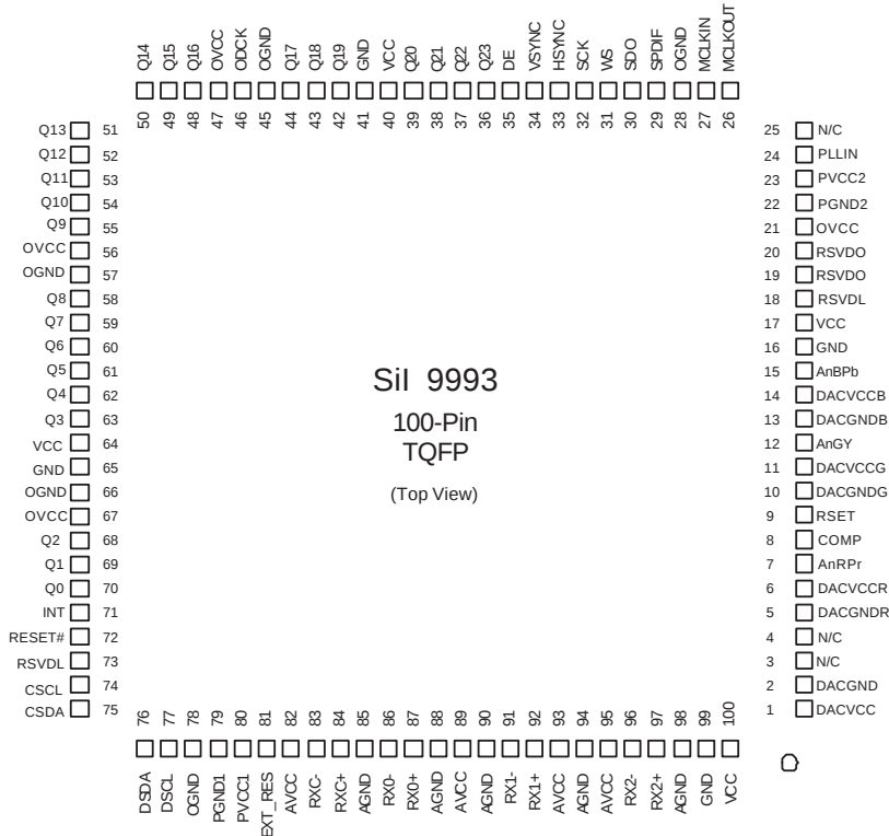
Figure 9-7 Internal Block Diagram and Pin Configuration
