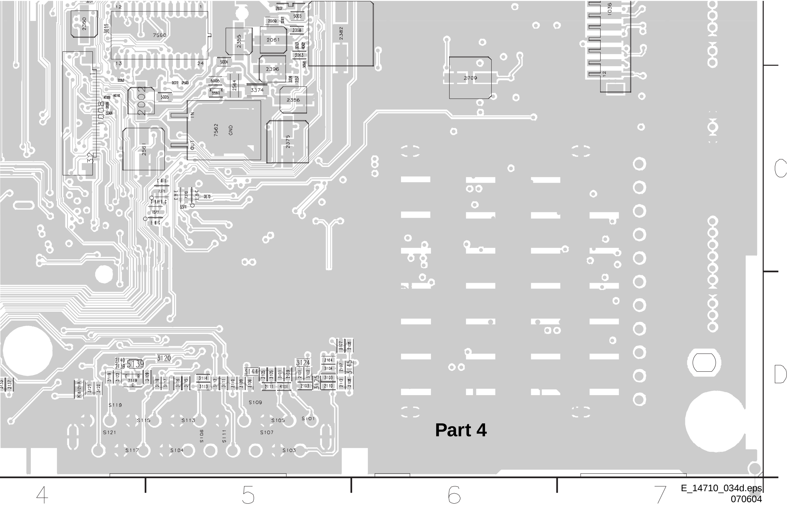
Layout Small Signal Panel (Top Side Part 4)
