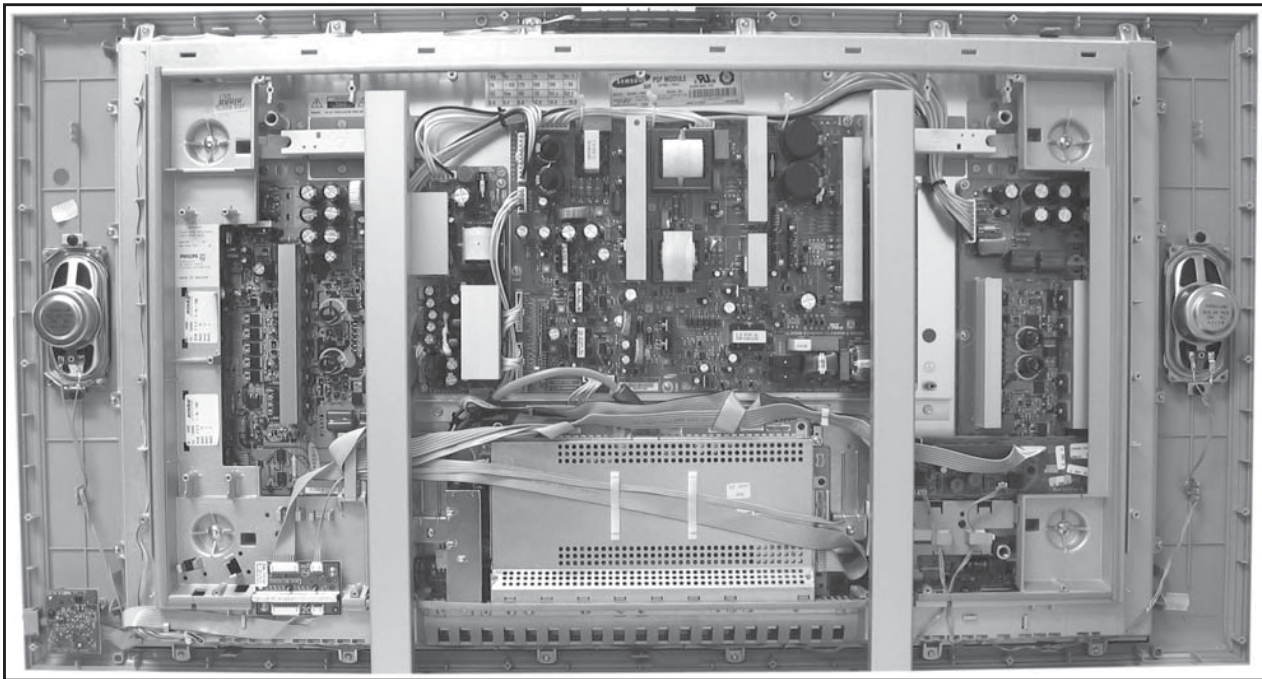
Figure 4-1 Cable dressing
