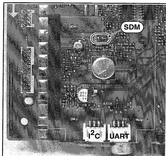
Figure 5-1 SDM Service jumper
