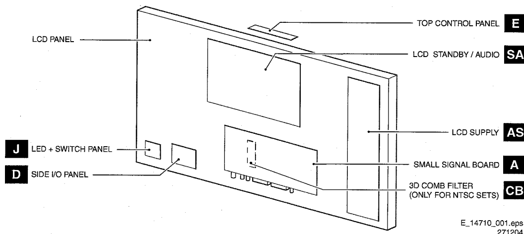
Figure 1-5 Chassis Overview
