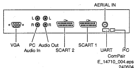
Figure 1-1 Rear connections
