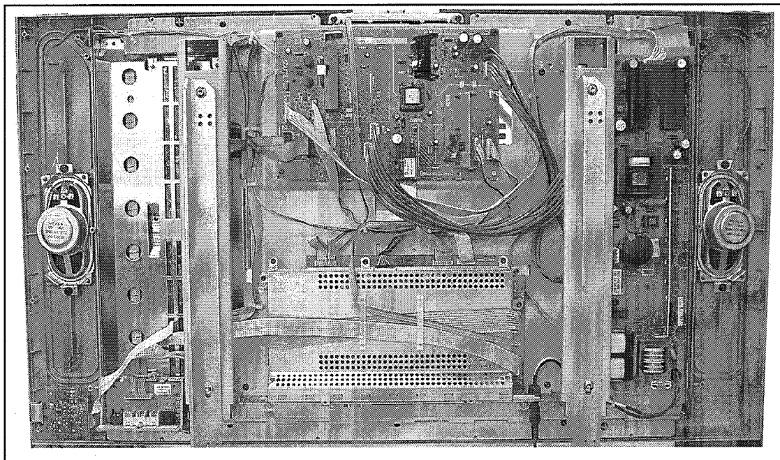
Figure 4-1 Cable dressing
