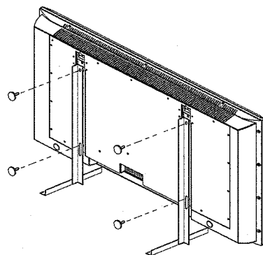
Figure 4-3 Aluminium stands
