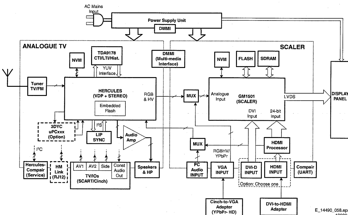
Figure 9-1 Block Diagram
