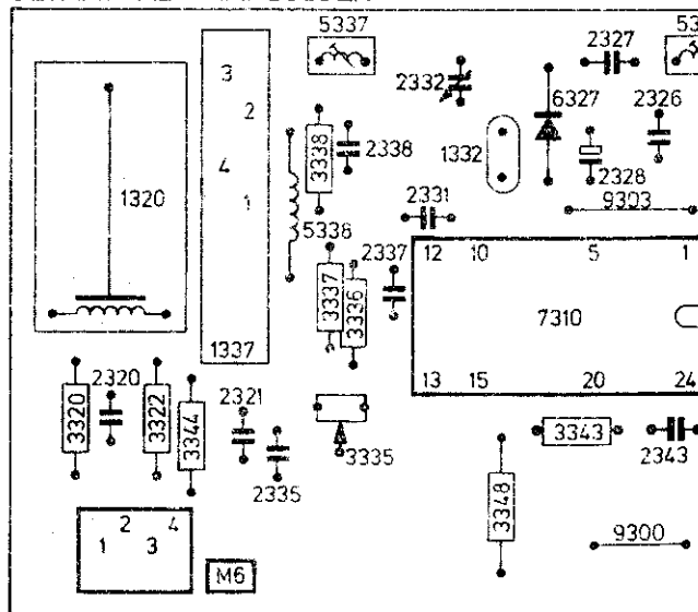
SECAM/PAL TRANSCODER
