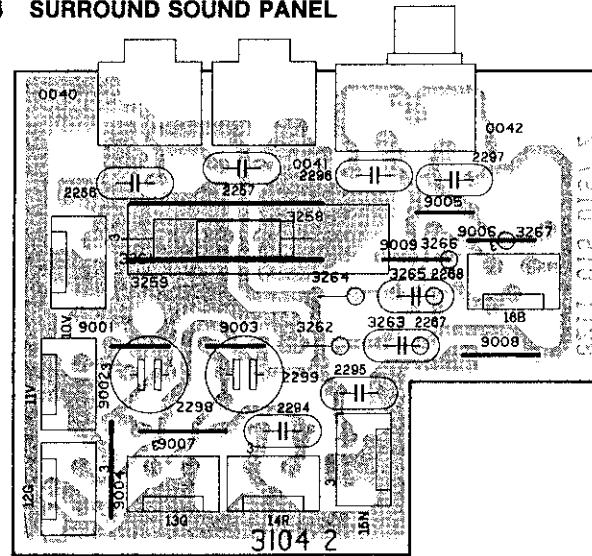
1004 SURROUND SOUND PANEL
