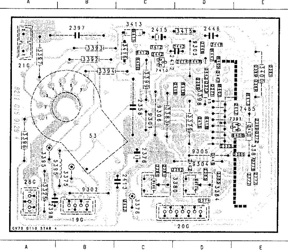
1002 PICTURE TUBE PANEL
