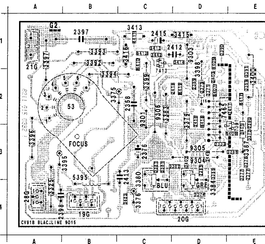
1005 PICTURE TUBE PANEL BLACKLINE
