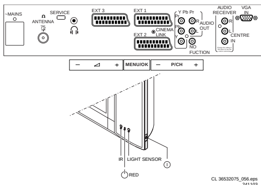
Figure 1-1 Rear/Bottom connections
