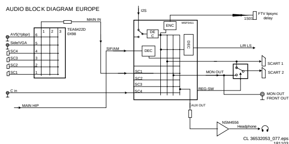
Figure 9-7 Audio block diagram
