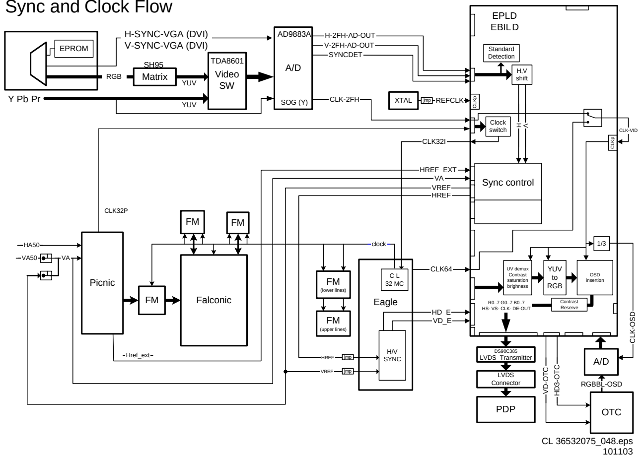
Figure 9-11 Sync and clock flow
