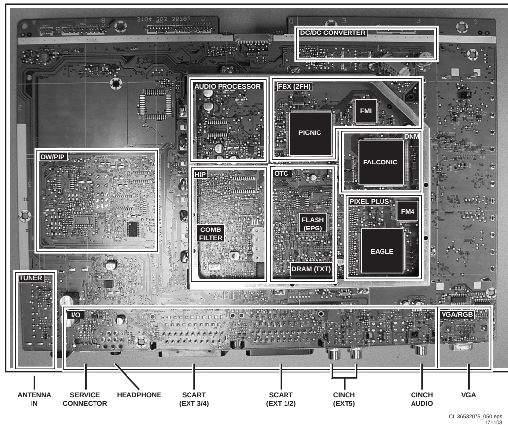
Figure 9-2 SSP bottom view
