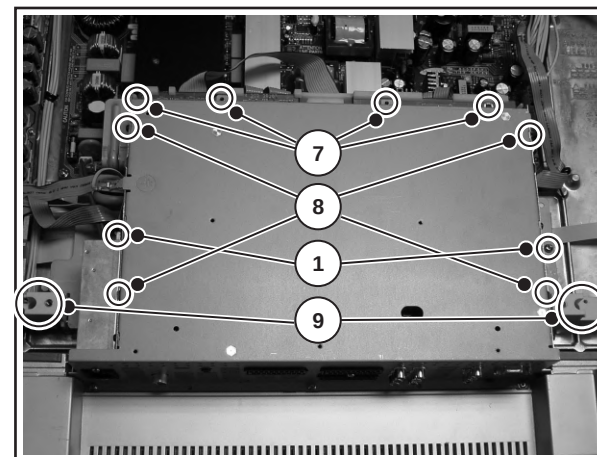
Figure 4-4 SSB Box. Top view
