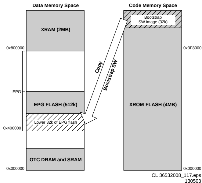
Figure 9-14 Memory diagram (initial situation)
