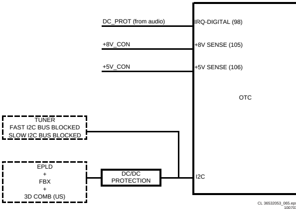
Figure 5-4 Protection diagram.
