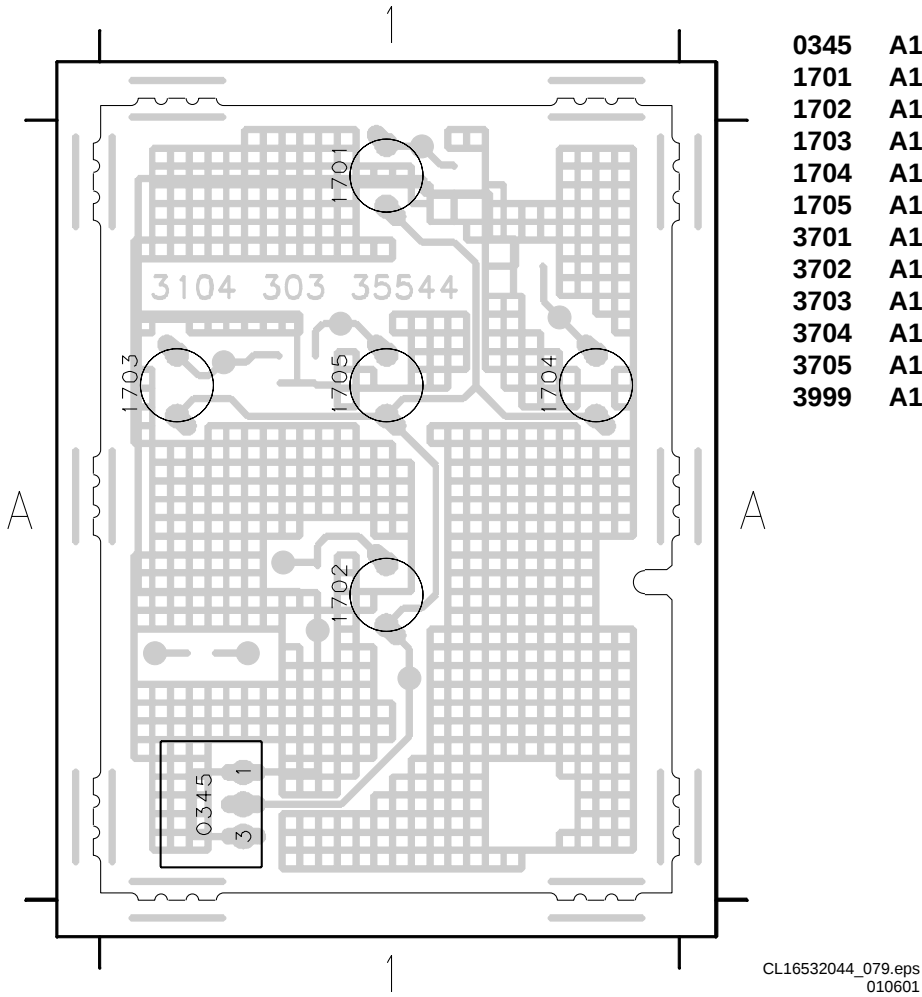
Layout Top Control Panel (Bottom Side)
