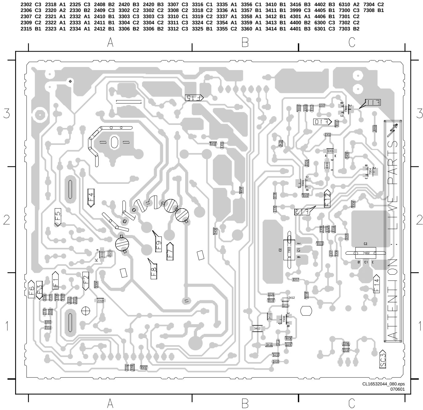
CRT/SCAVEM Panel (Bottom Side)
