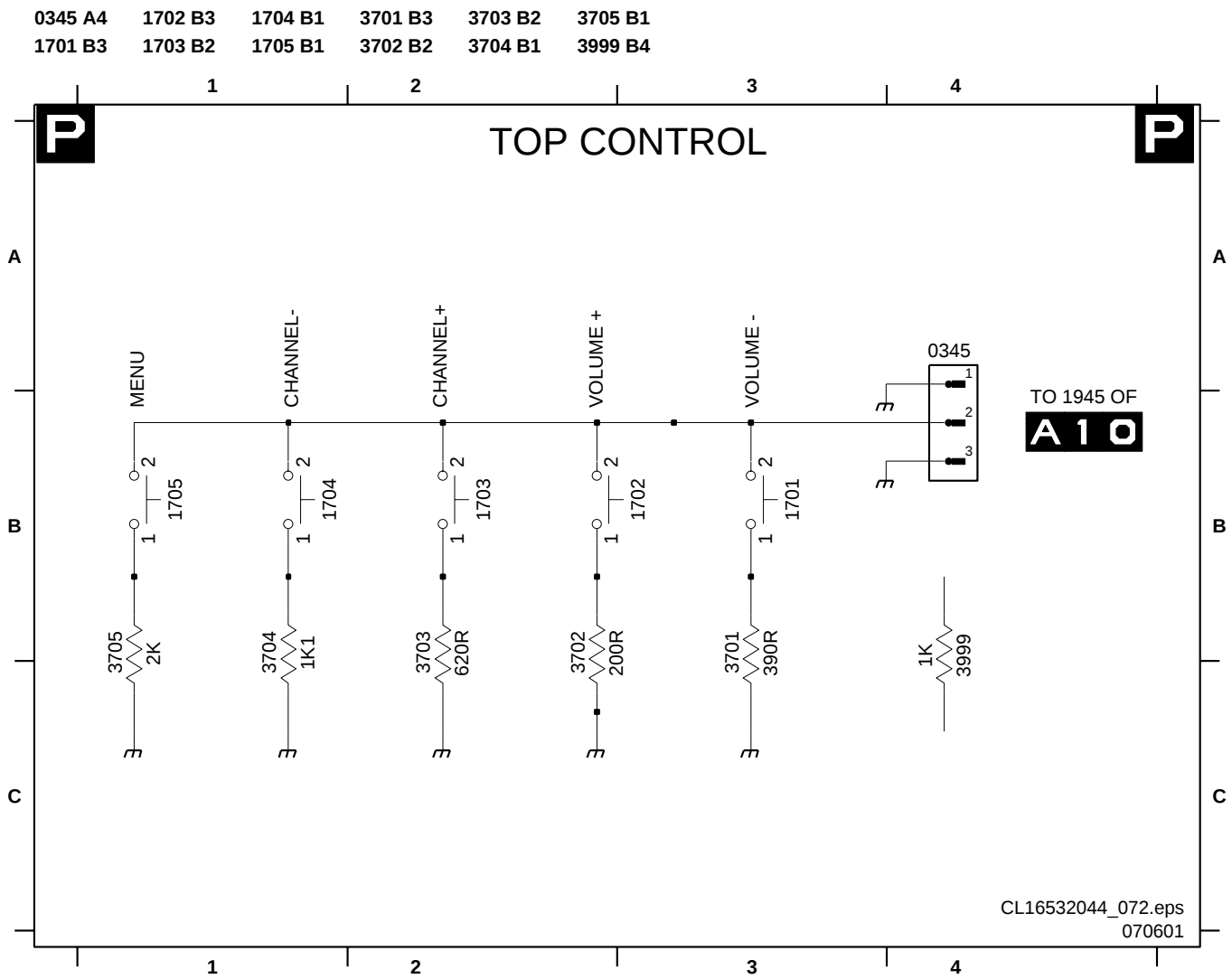
Top Control Panel
