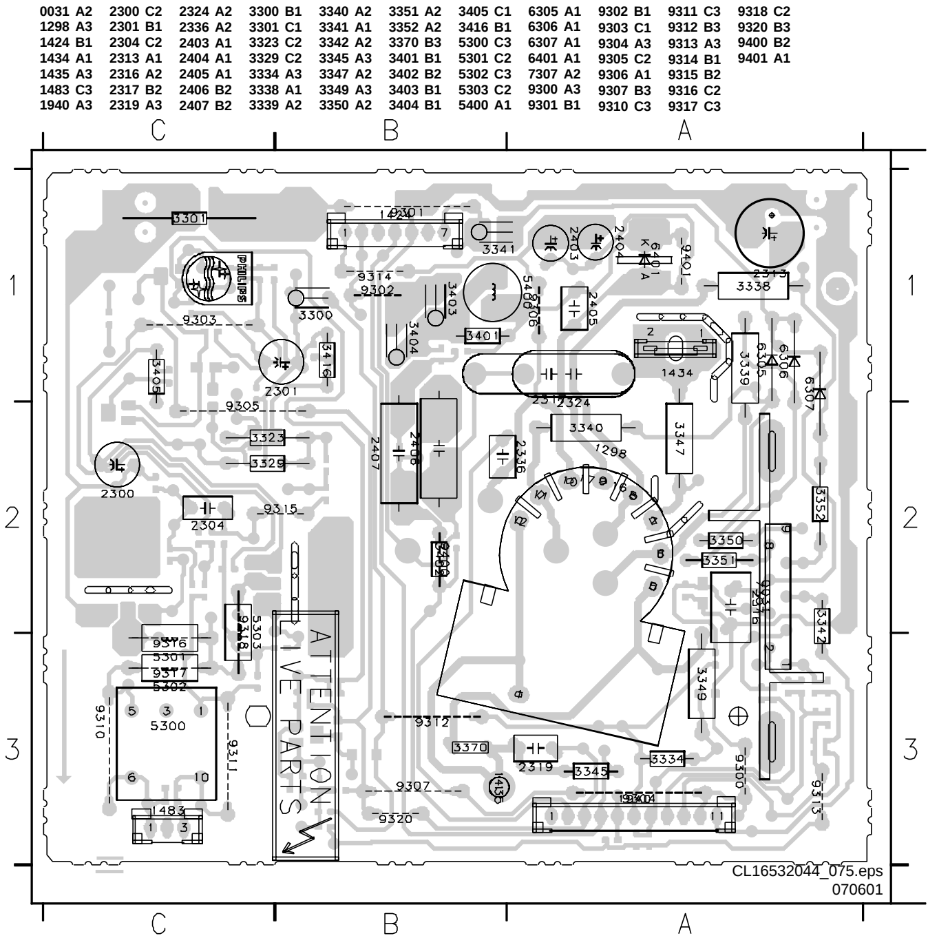
CRT/SCAVEM Panel (Top Side)
