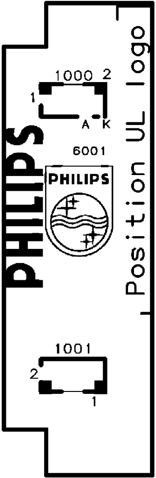
CBA Layout (Top View)
