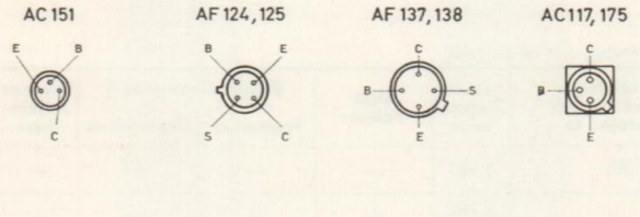
TRANSISTORANSCHLÜSSE TRANSISTOR TERMINALS
