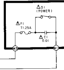
G AC IN CIRCUIT
