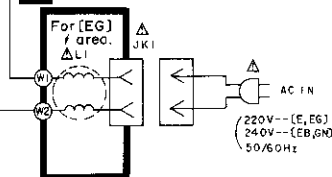
G AC IN CIRCUIT
