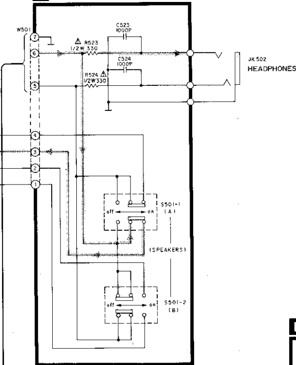
E HEADPHONES CIRCUIT
