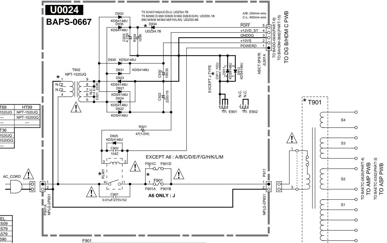
Model No. TX-NR509/609/HT-R690/990/HT-RC360 Schematic Diagram (Part-10) PS Section
