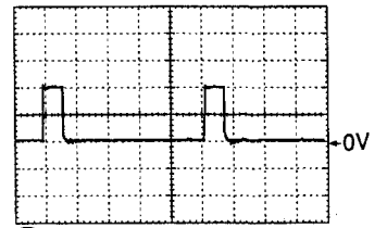
③ 5V/cm, 5µs/cm
