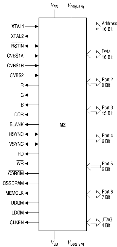
Pin Diagram (top view)
