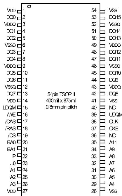
Pin Configuration
