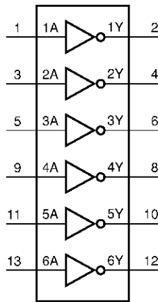
Logic symbol.
