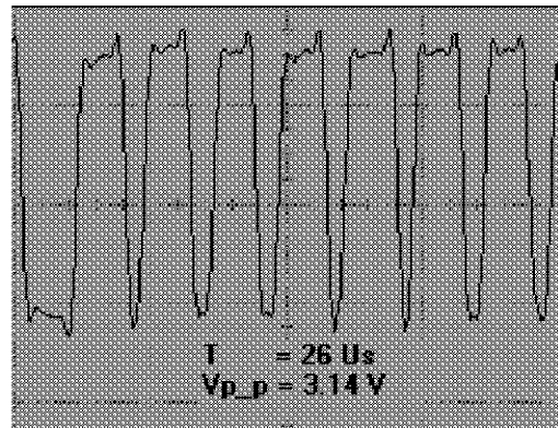
SCL 3_3 X204 PIN (17)
