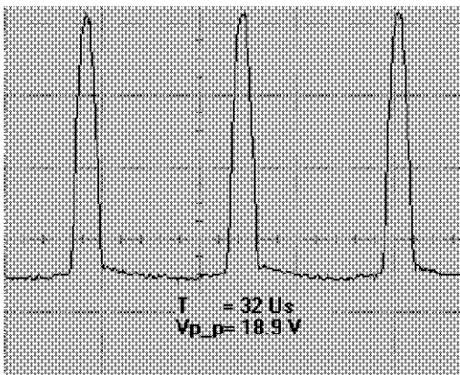
FLY_BACK X205 PIN (2)
