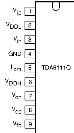
Pin configuration.
