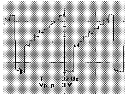
GREEN X701 PIN (4)
