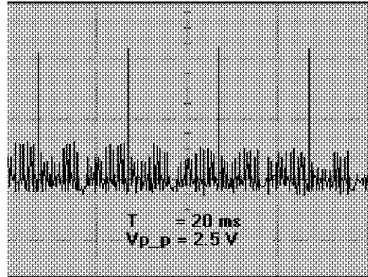
CUT OFF X701 PIN (10)
