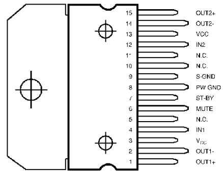
PIN CONNECTION
