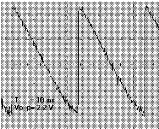
V_DRIVE (-) X205 PIN (5)
