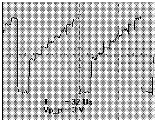
RED X701 PIN (2)
