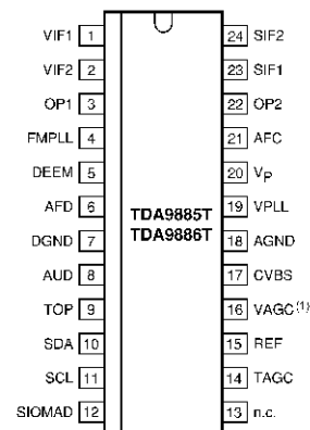
Pin configuration
