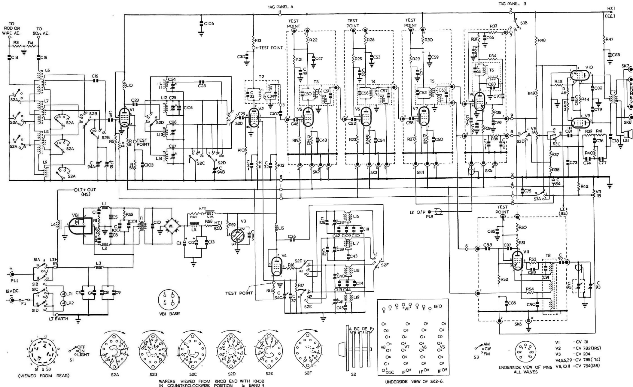
Fig. 3. Circuit Diagram of Reception Set R209 Mk. II.
