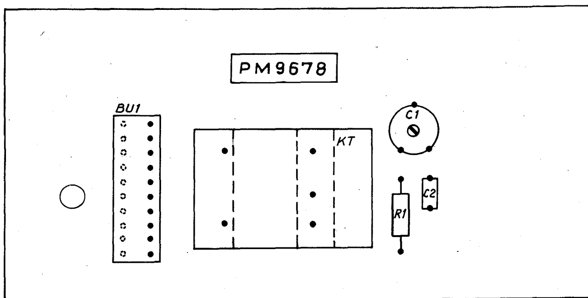
Figure VIII-3. Component lay-out PM 9678
