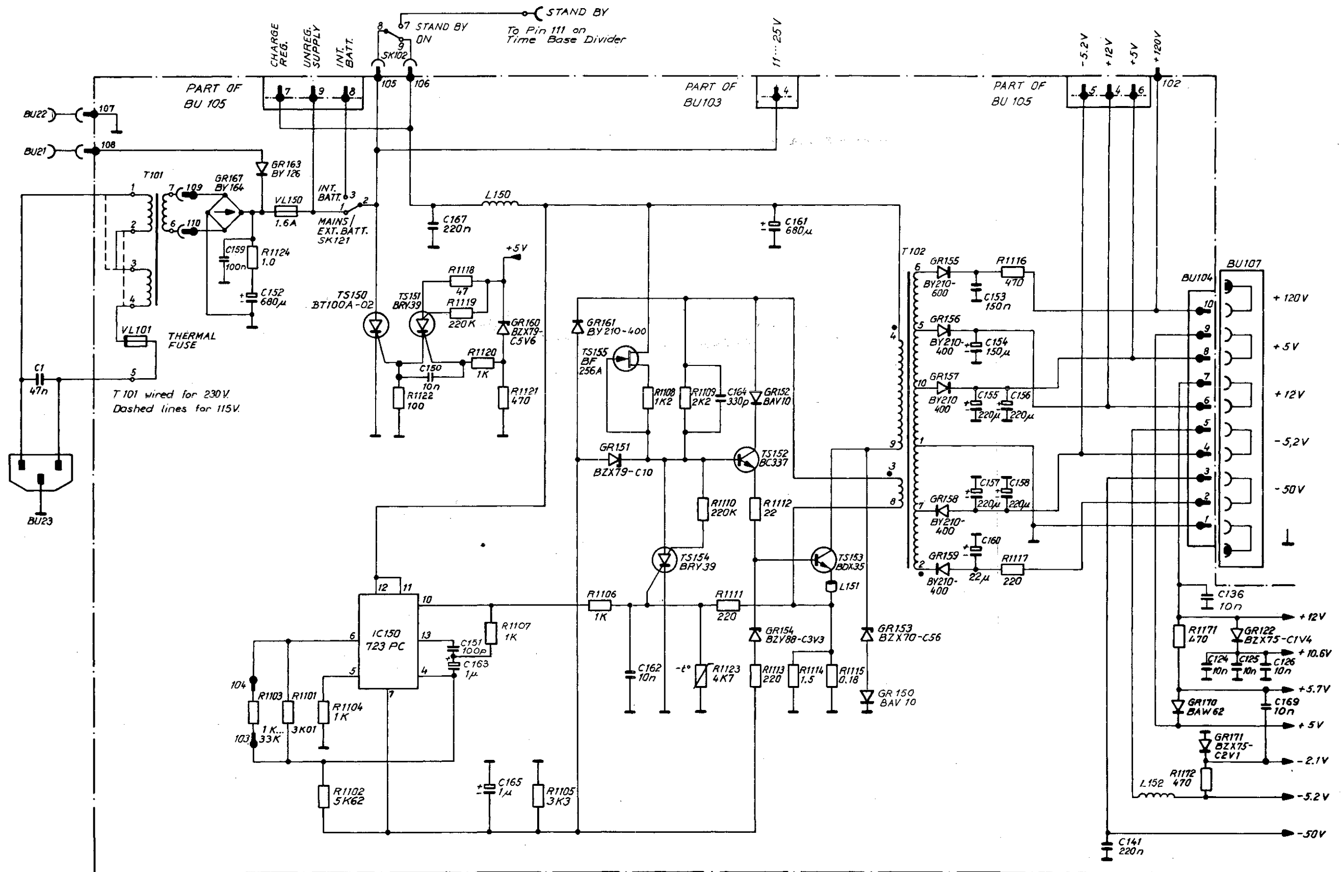
Figure X-5. Power supply
