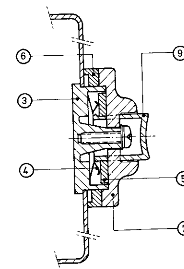
Fig. 15 Handle: spare parts
