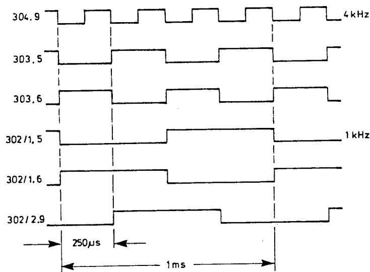
Fig.5 Generation of the 1 kHz signals
