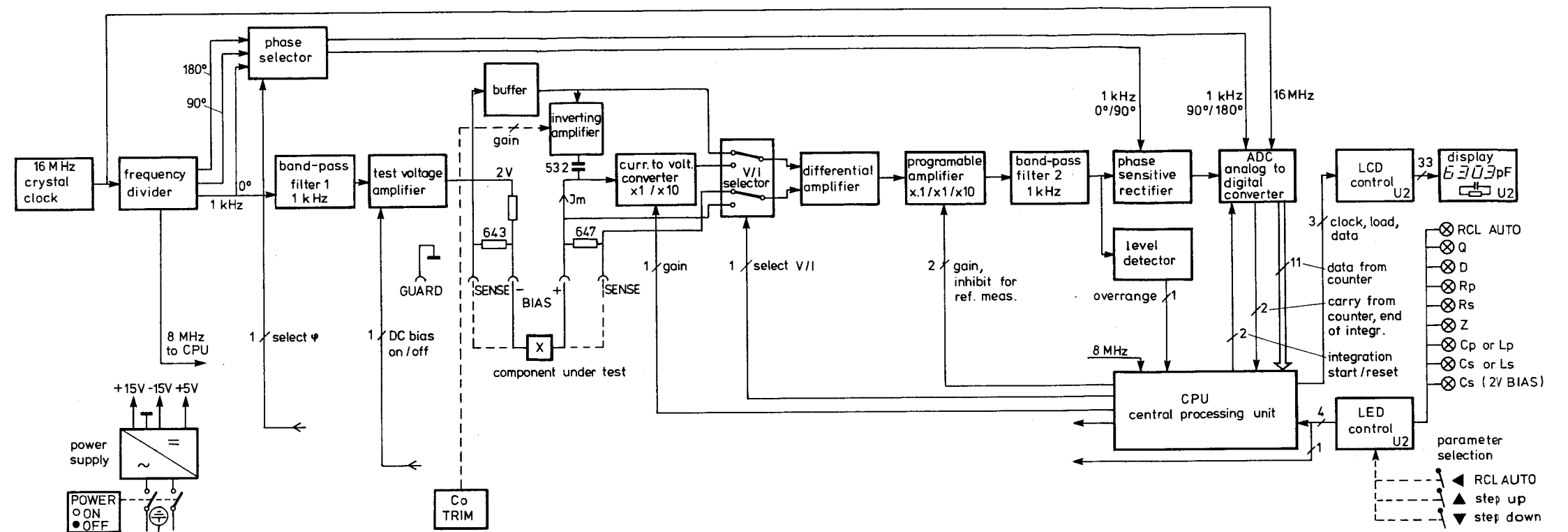
Fig. 3 Block diagram
