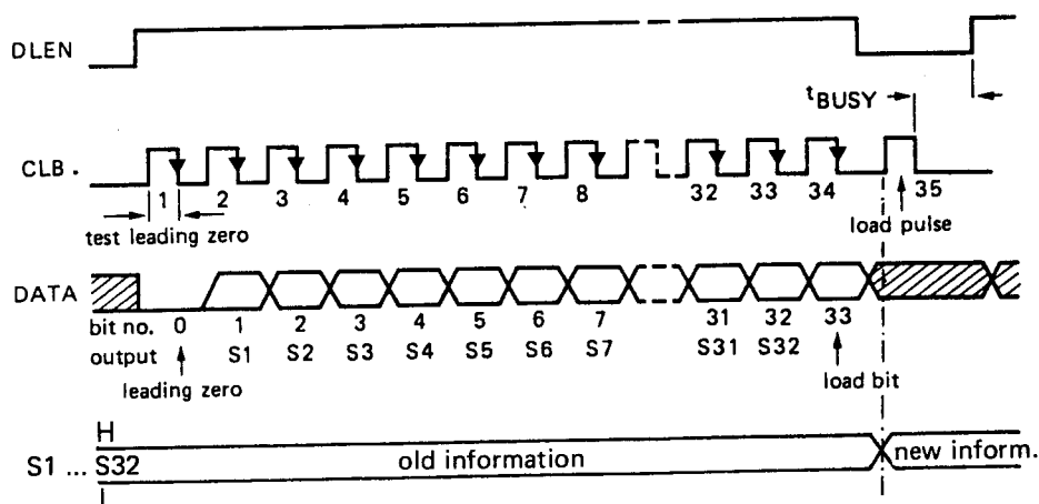
Fig. 9 Data format microprocessor (unit 1)/display driver (351, unit 2)
