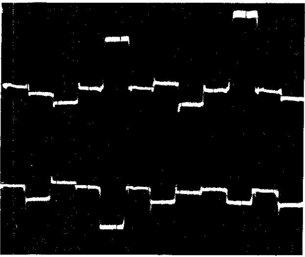
Fig. 33. Pattern of colour definition lines and saturation steps combined
