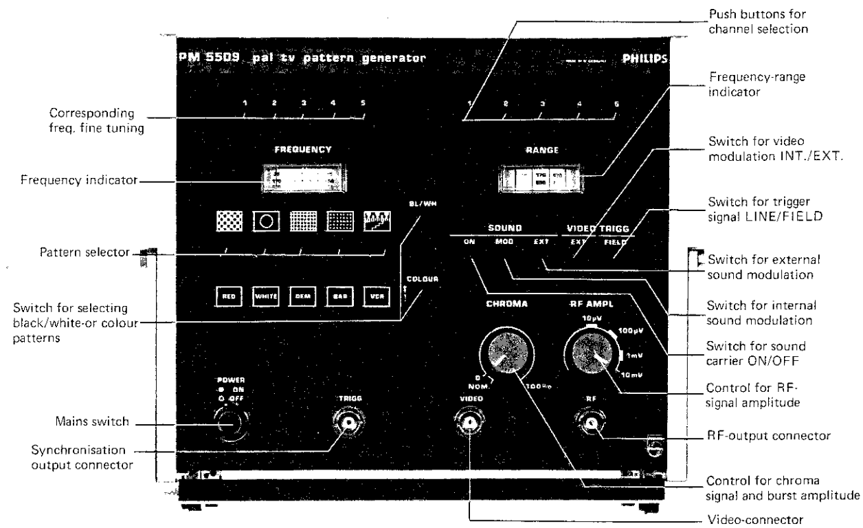
Fig. 1. Front view, controls and sockets
