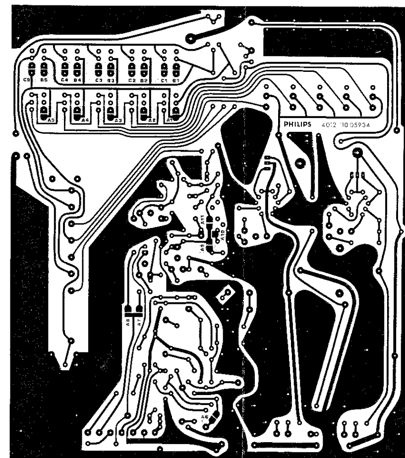
Fig. 4. Printed wiring, unit 2
