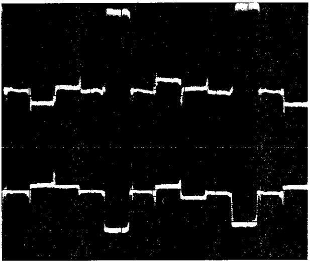
Fig. 31. Correct (G-Y) signal (green-colour difference signal)
