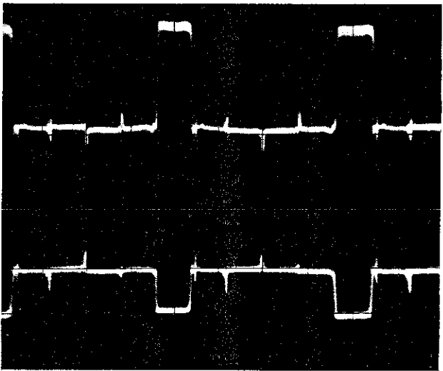
Fig. 34. Delay line and demodulators, correctly adjusted
