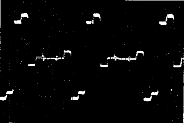
Fig. 29. Correct (R-Y) signal (red-colour difference signal)
