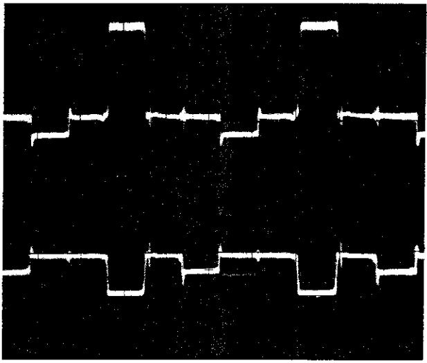
Fig. 38. Demodulators, general-phase fault
