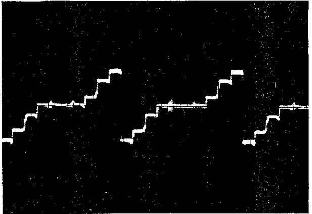
Fig. 31. Correct (G-Y) signal (green-colour difference signal)
