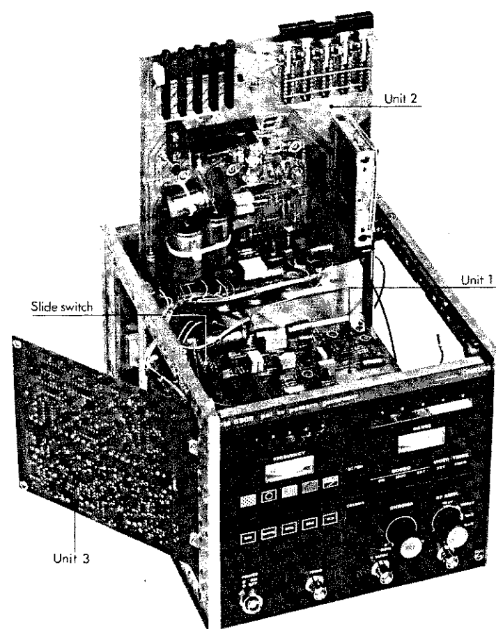
Fig. 6. Exploded view
