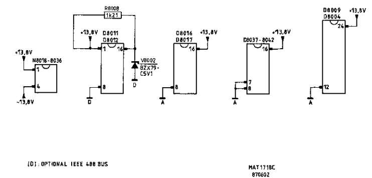
Fig.9.3. IEEE 488 bus unit, circuit diagram 2 (analog part)
