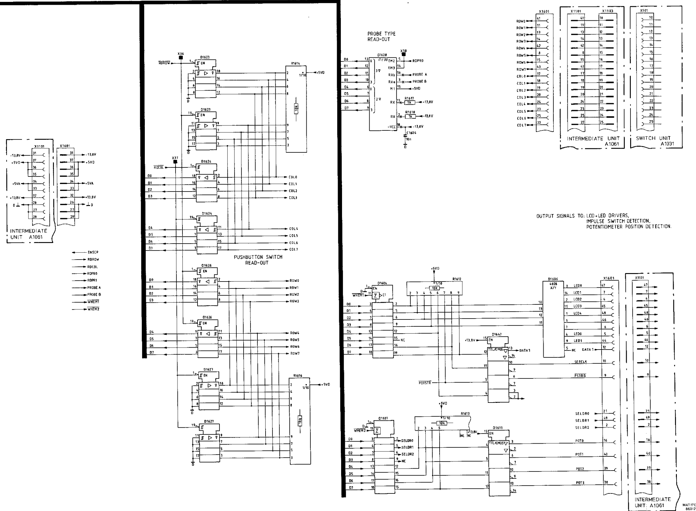
Fig.7.6. Central processor unit, circuit diagram 3.
