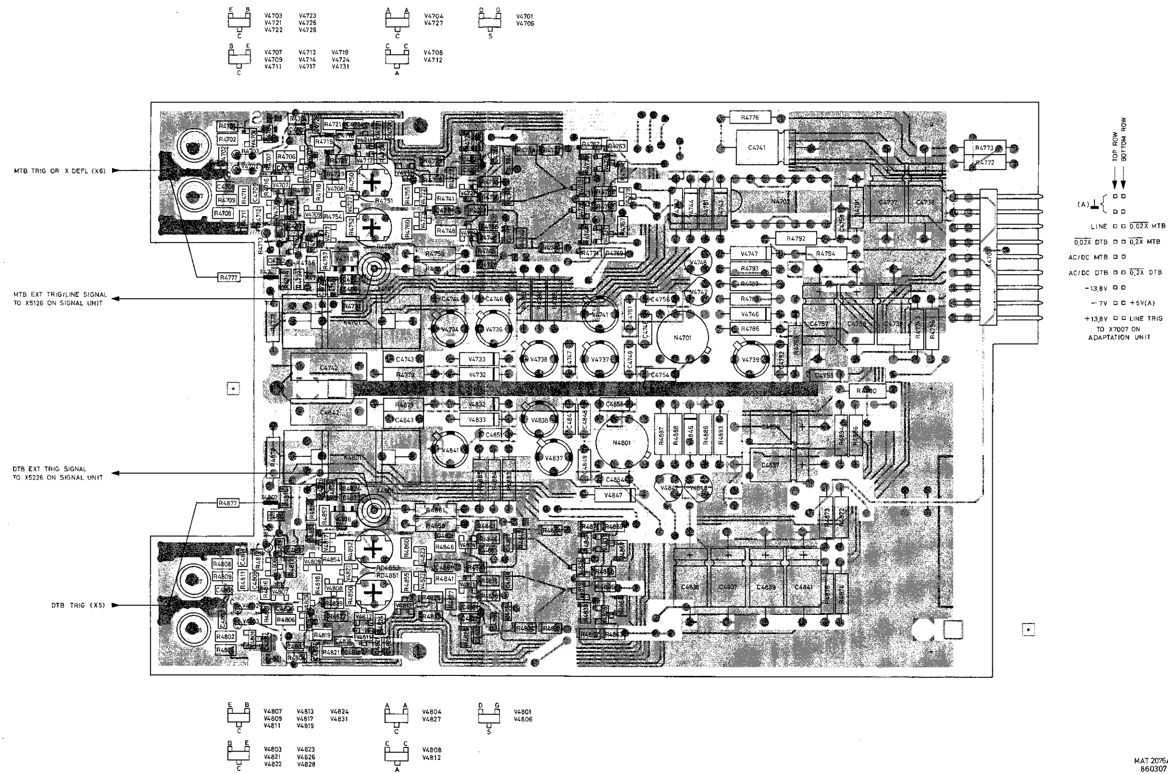
Fig.11.1. External MTB/DTB trigger unit, p.c.b. lay-out.
