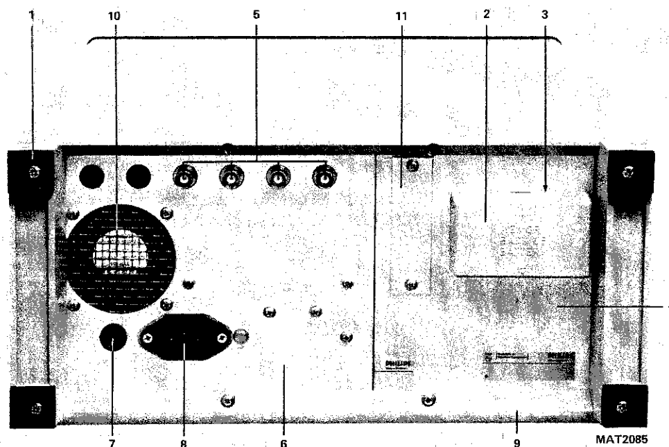
Fig. 28.2 Mechanical parts REAR SIDE
