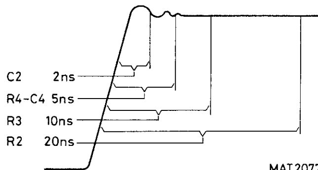
Fig. 29.3 Adjusting elements
