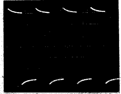
Fig.29.2.c Under compensation
