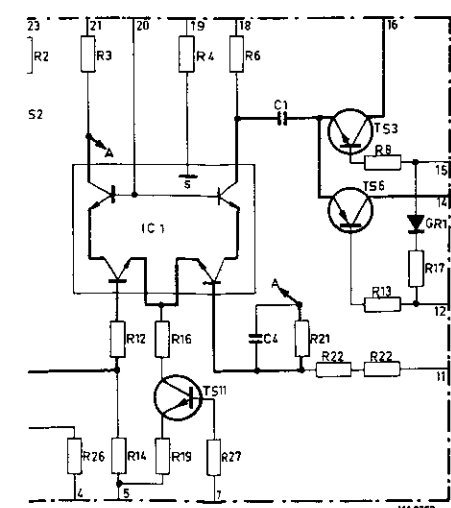
n trigger-pulse shaper (hybrid circuit)
