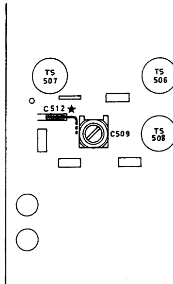
Fig. 1. Increasing p.c. capacitance C512
