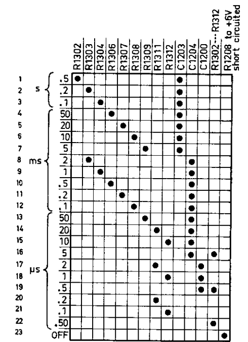
Fig. 3.56. Table of TIME/DIV switch positions
