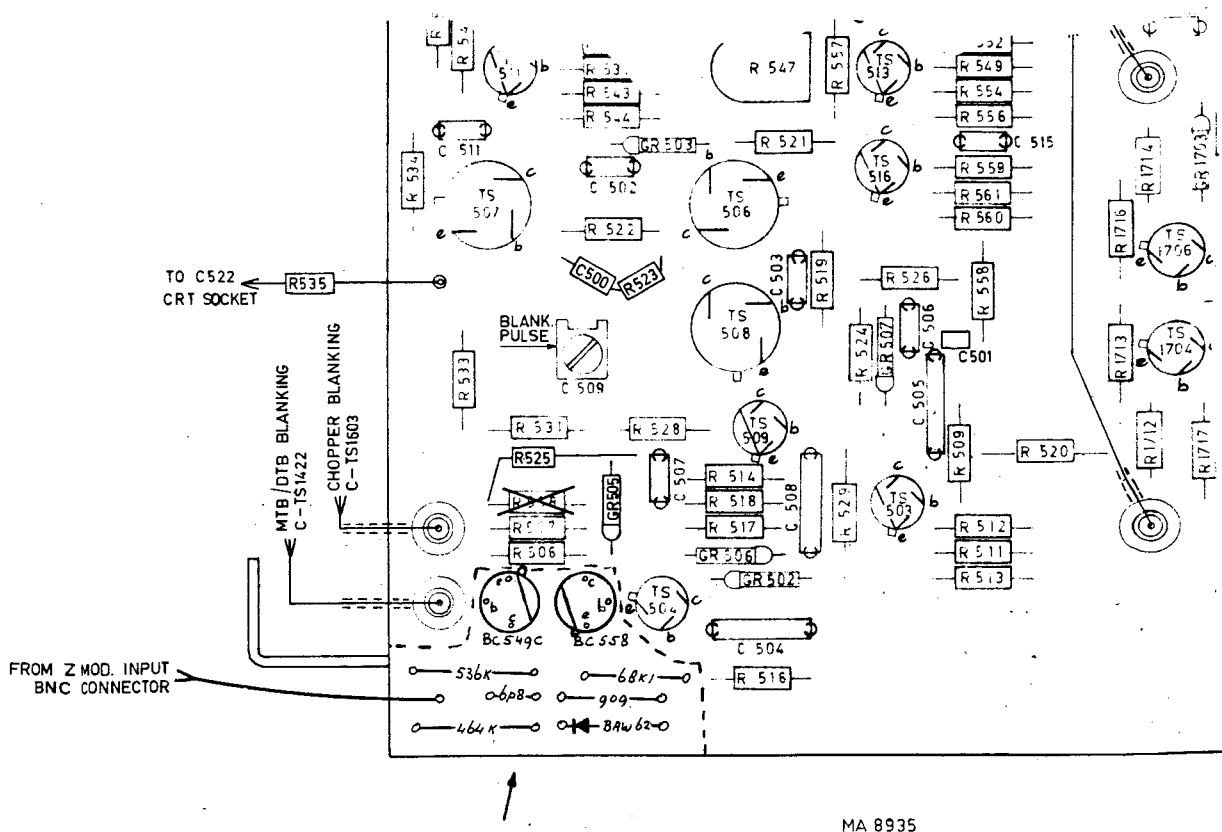
Fig. 2. Component lay-out additional ext. Z mod. circuit.
