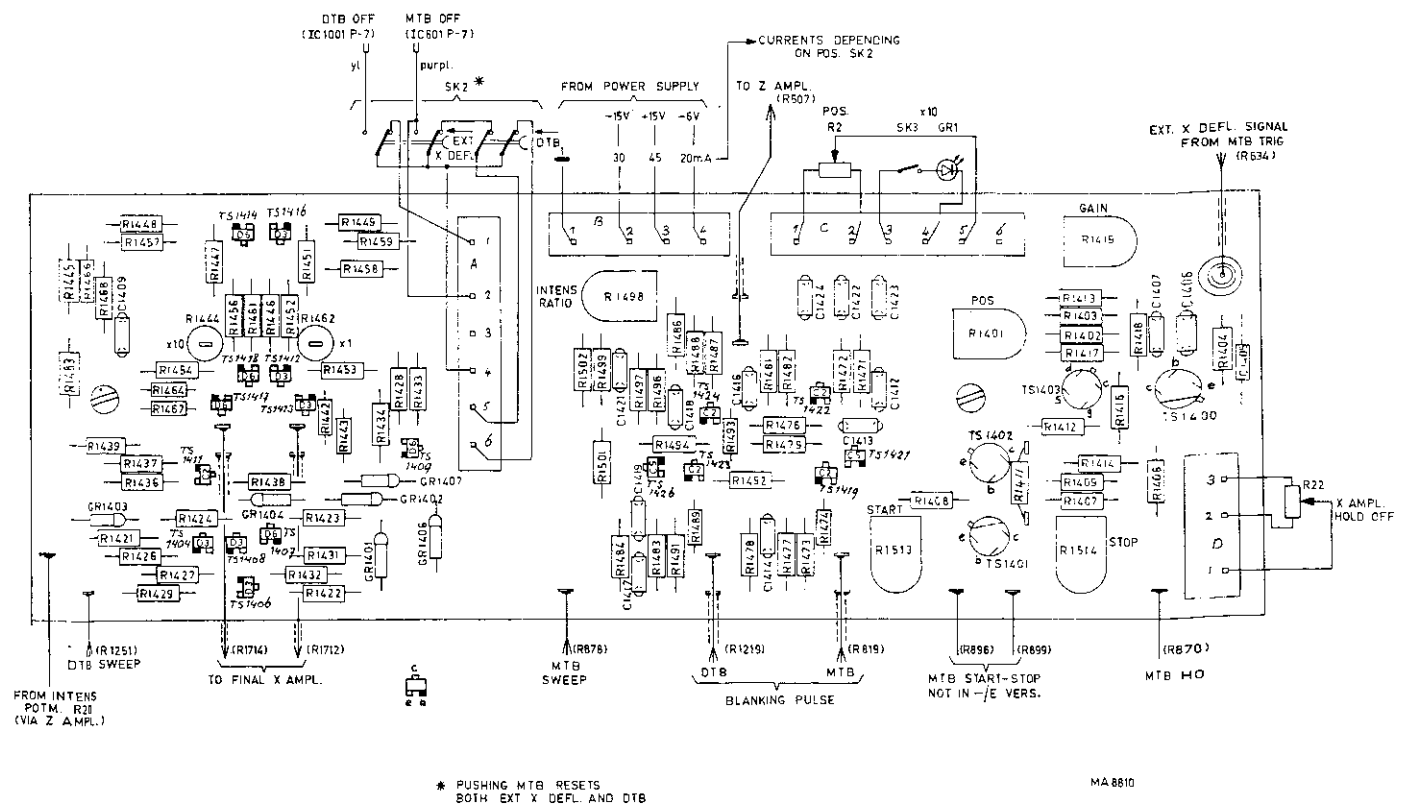
Fig. 3.59. X Deflection selector board PM 3260/02
