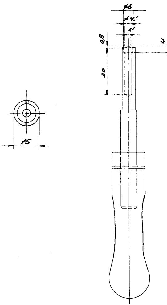
Fig. 3.10. Tool for positioning potentiometer
