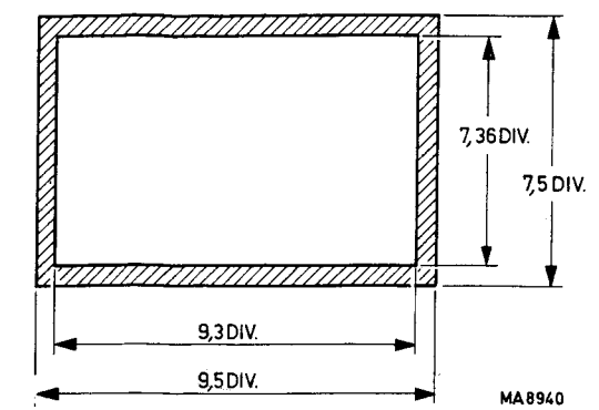
Fig. 3.17. Geometry check
