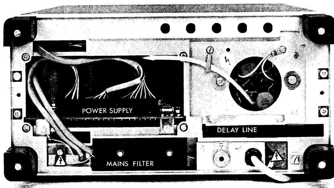
Fig. 3.30. Rear view without rear plate
