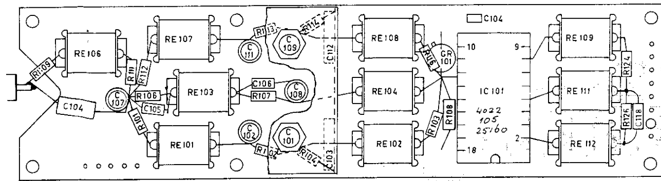
Fig. 3.34. Y Attenuator circuit board
