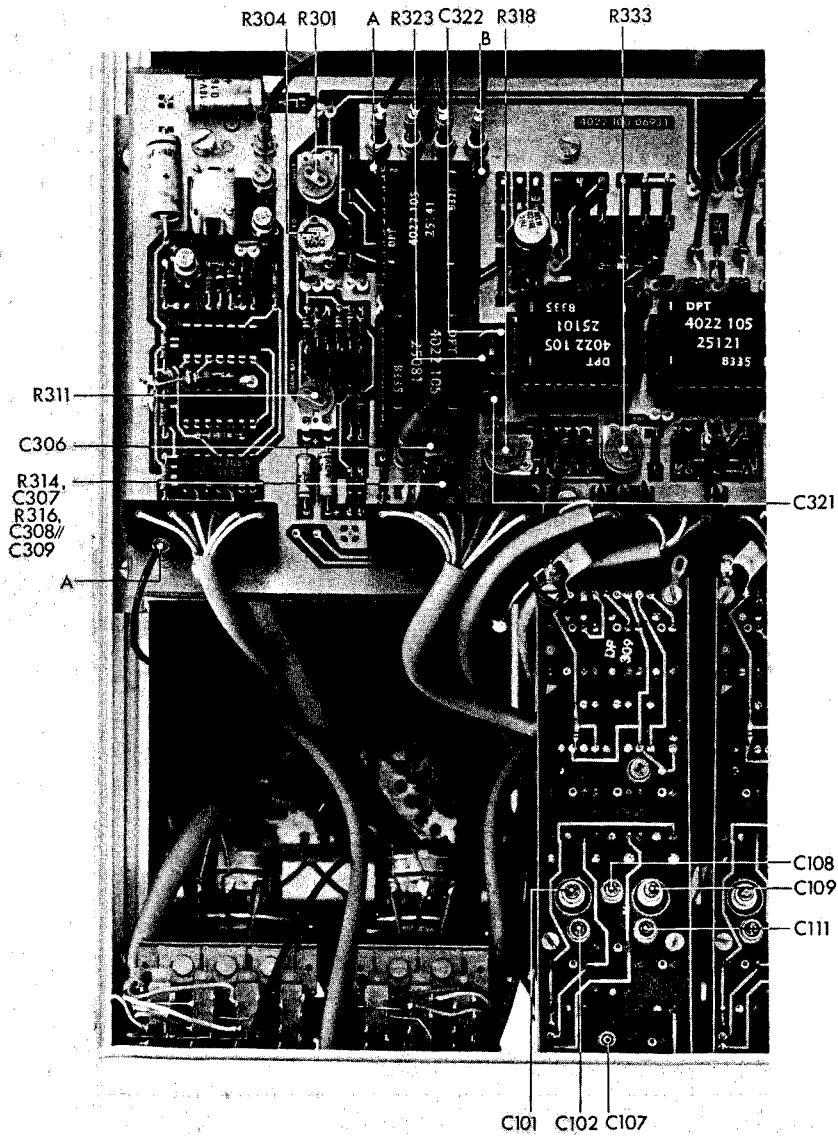
Fig. 3.18. Intermediate amplifier board with adjusting references
