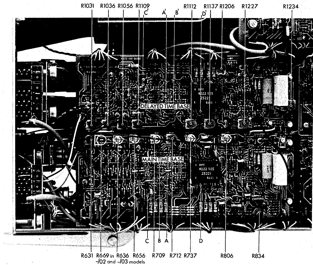
Fig. 3.22. Time-base boards with adjusting references
