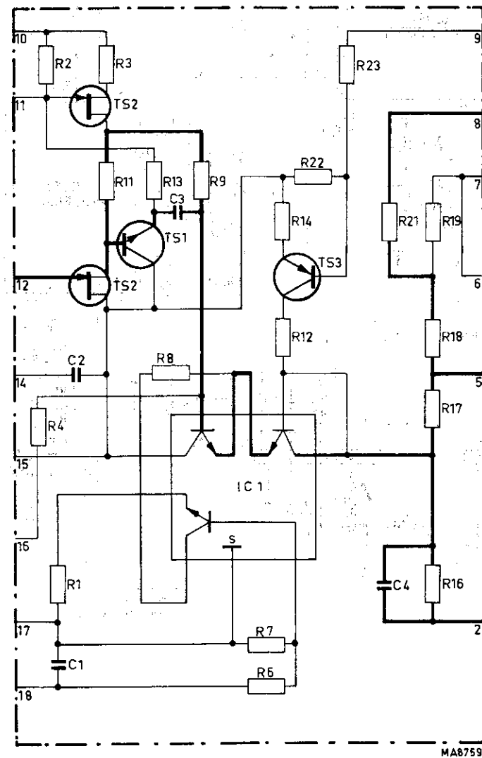
Fig. 3.35. Circuit diagram impedance converter (hybrid circuit)
