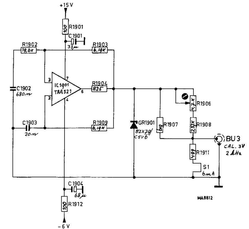
Fig. 3.65. Calibration circuit diagram
