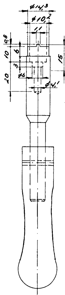
Fig. 3.9. Tool for attenuator unit
