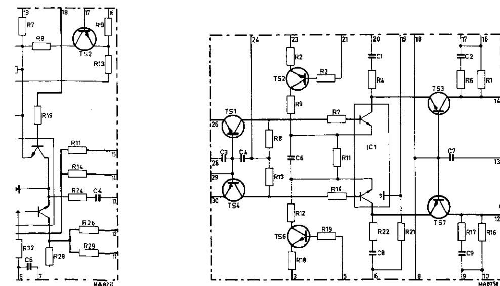
Fig. 3.45. Circuit diagram final amplifier (hybrid circuit)
