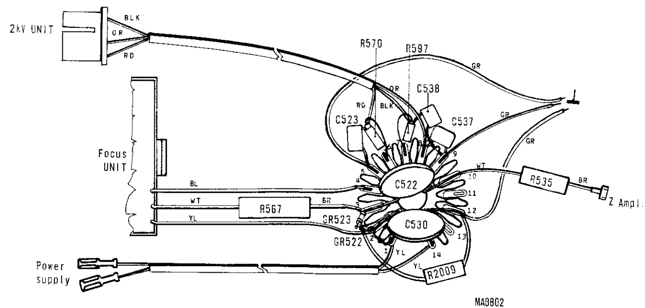
Fig. 3.64. C.r.t. socket assembly
