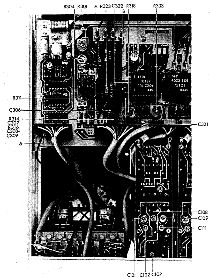
Fig. 3.18. Intermediate amplifier board with adjusting references
