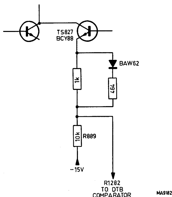
Fig. 2. Temperature drift compensation delay-time starting point
