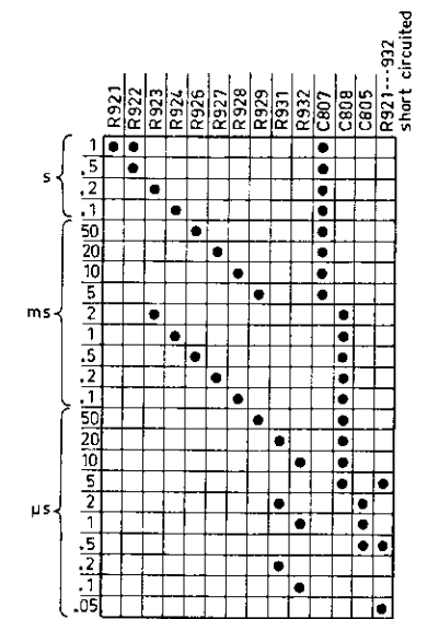
Fig. 3.51. Table of TIME/DIV switch positions
