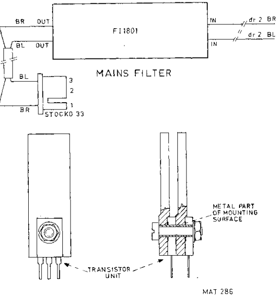
Fig. 3.40. Power supply p.c. board
