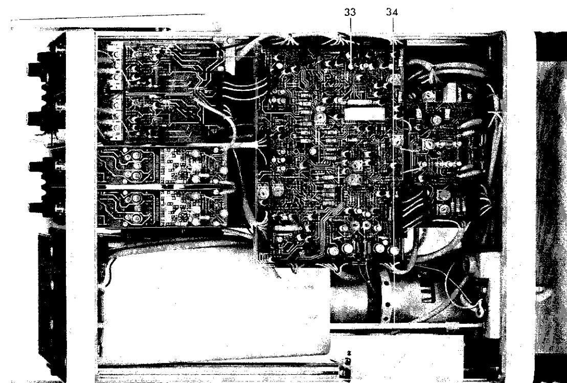
Fig. 3.18. Mechanical parts, bottom view
