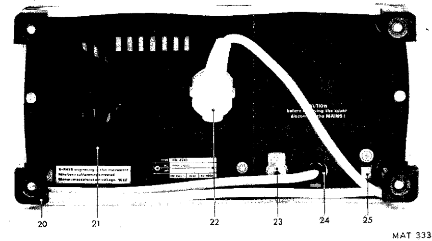
Fig. 3.16. Mechanical parts, rear view
