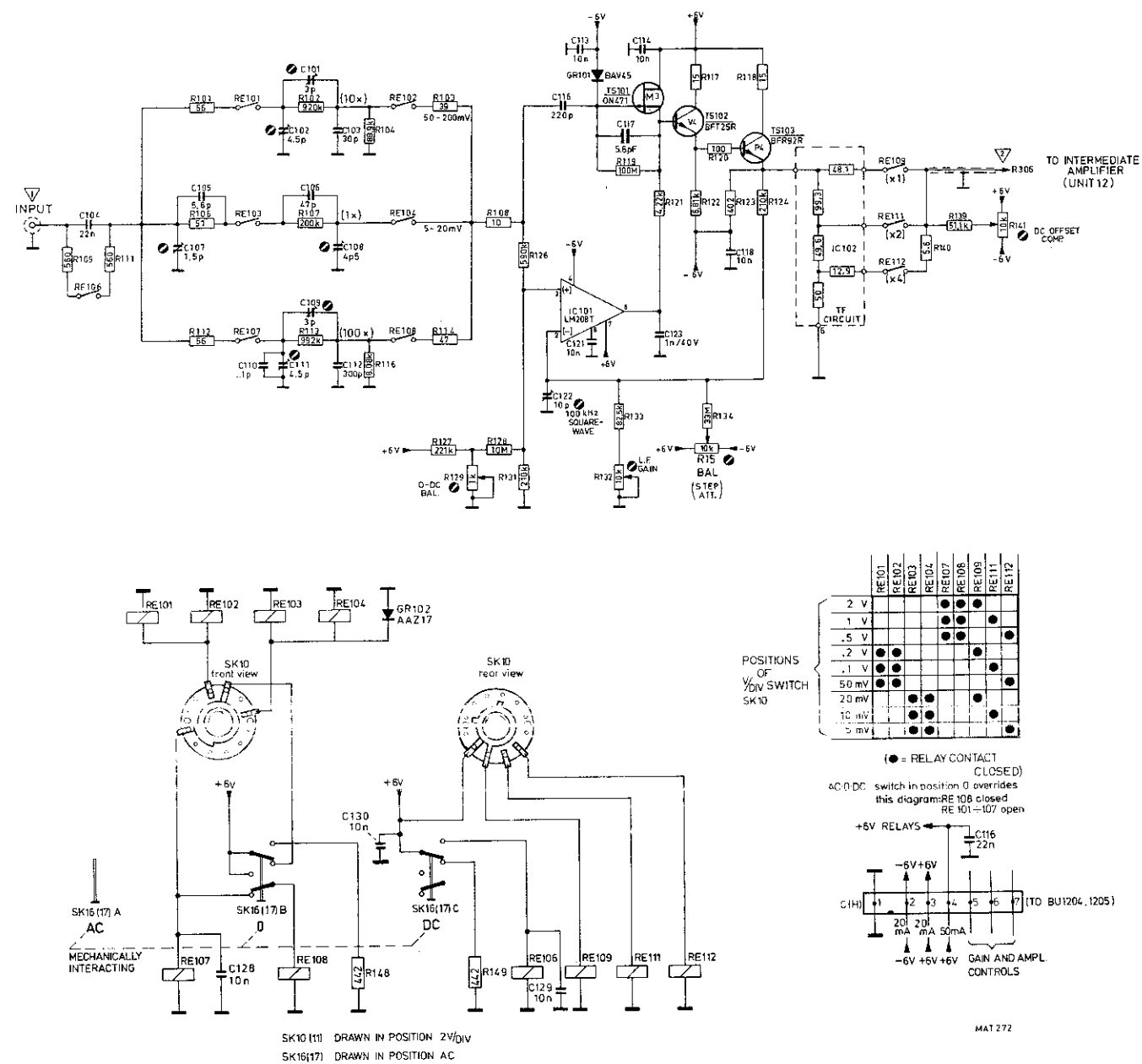
Fig. 3.21. Y-attenuator circuit diagram
