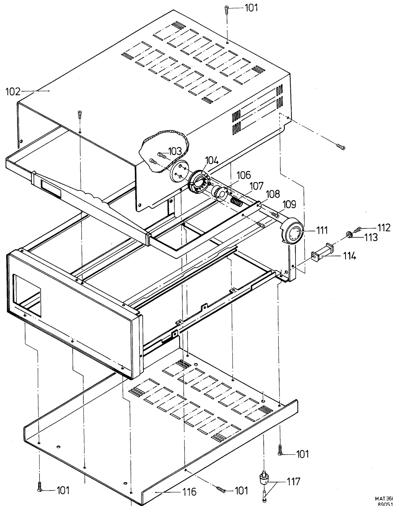
Figure 9.1 Housing
