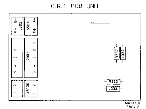
Figure 10.17 CRT pcb lay out
