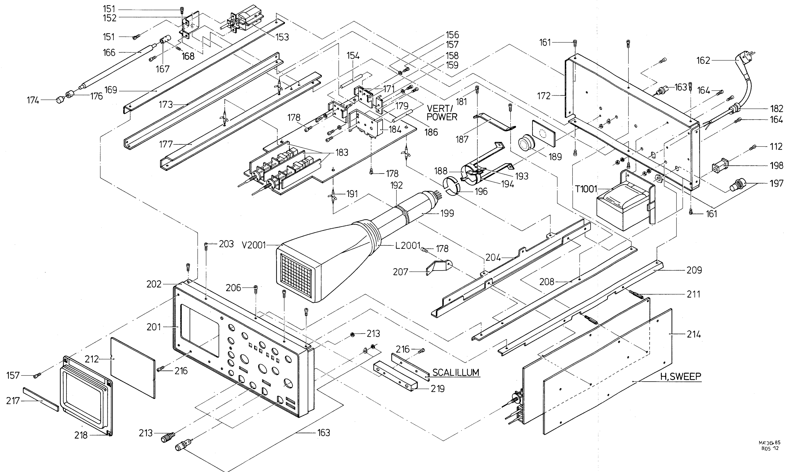
Figure 9.3 Main frame
