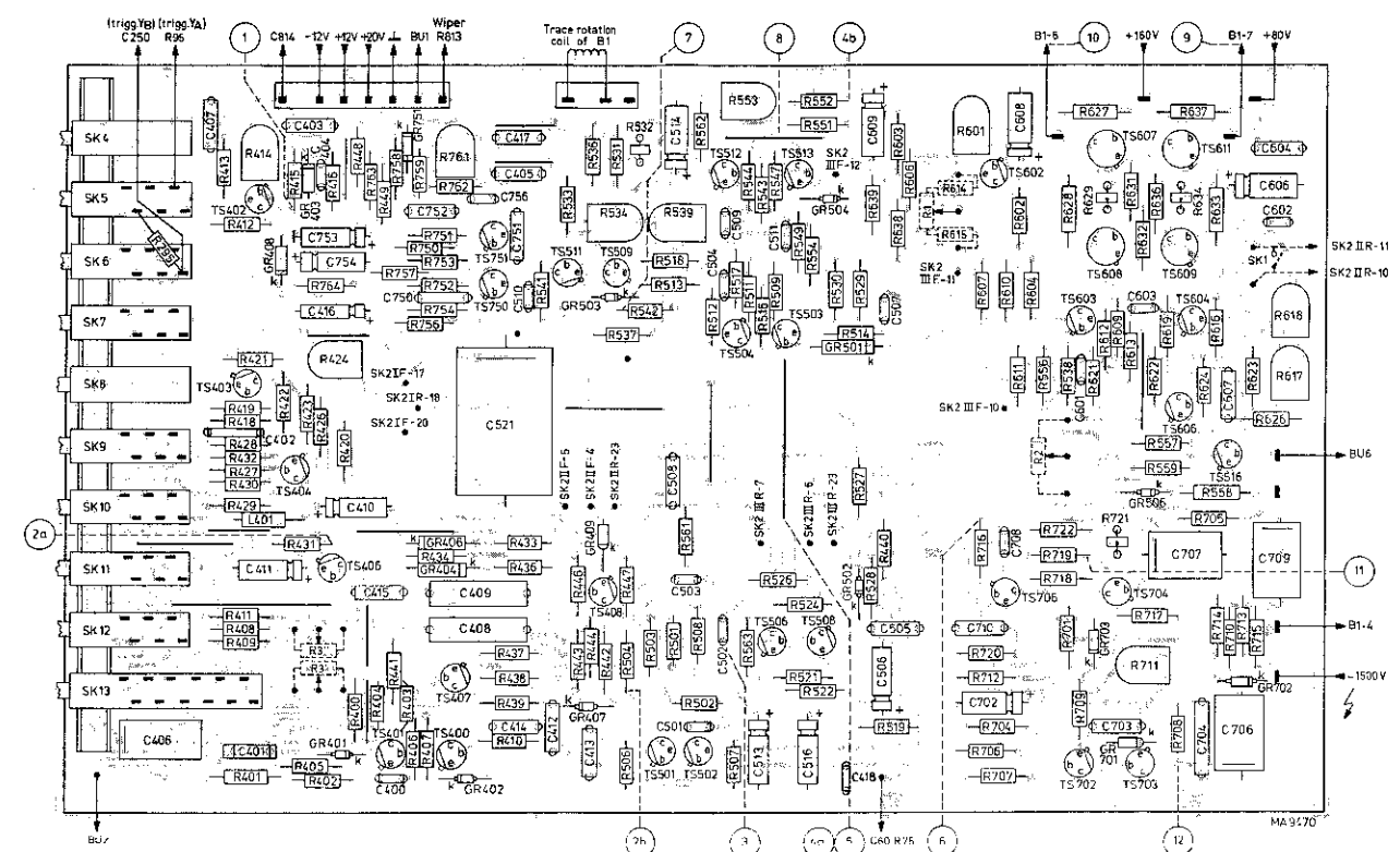
Fig. 3.41. Time-base unit
