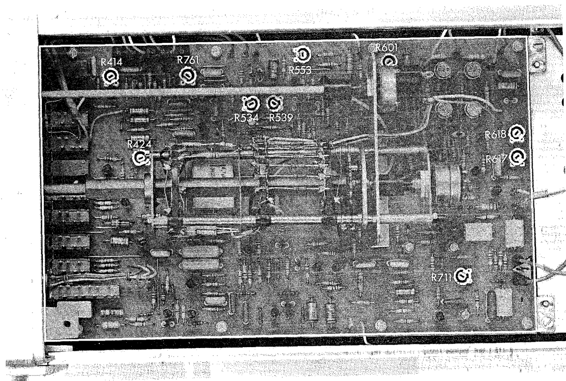
Fig. 3.12 Adjusting
