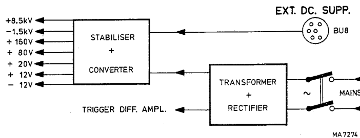
Fig. 3.8. Power supply
