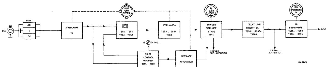
Fig. 3.1. Vertical amplifier, channel Y_A
