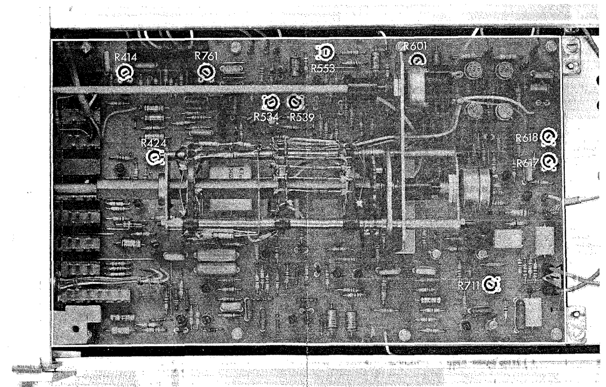
Fig. 3.12 Adjusting
