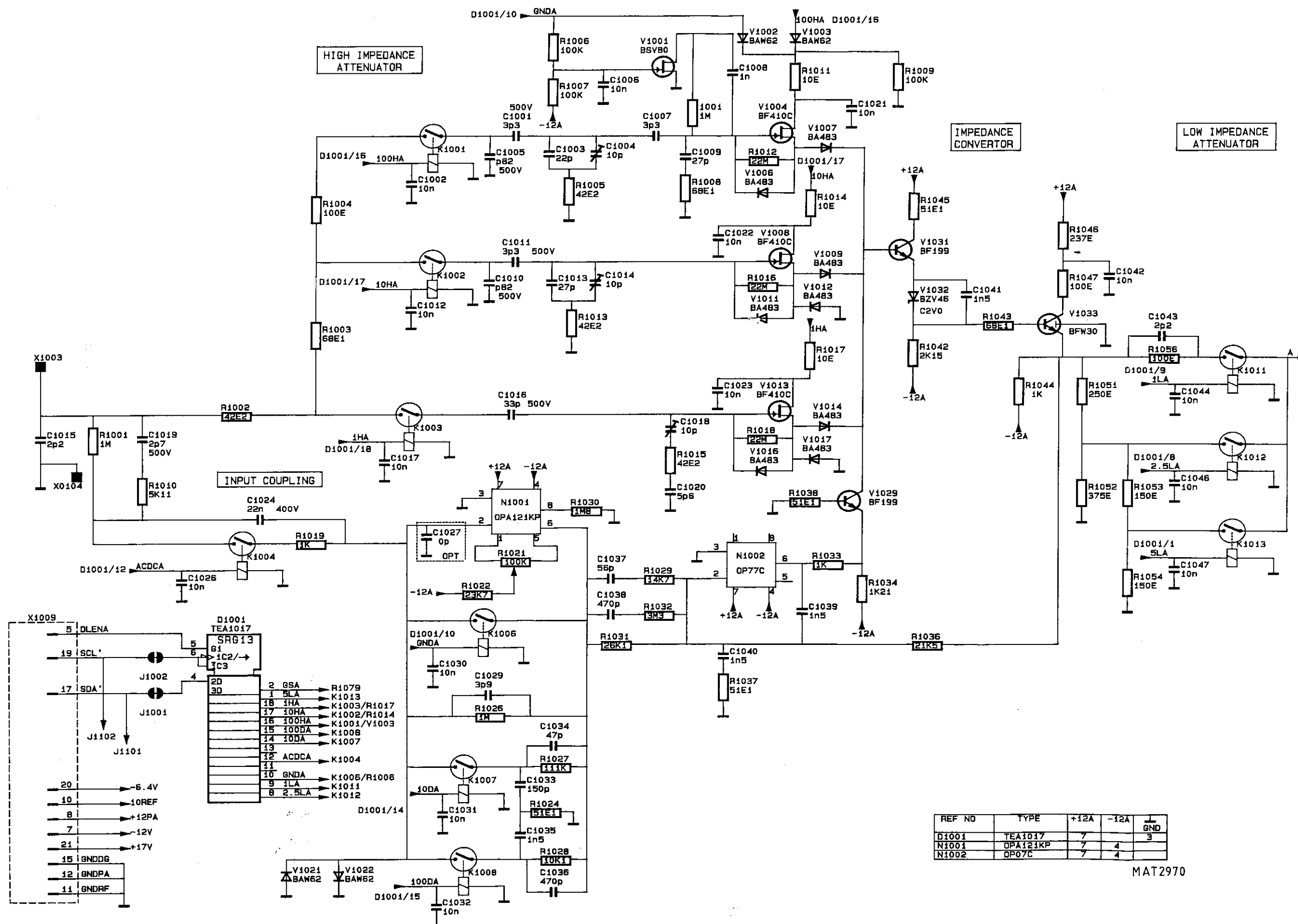
Figure 4.3 Circuit diagram of attenuator, ch. A 1
