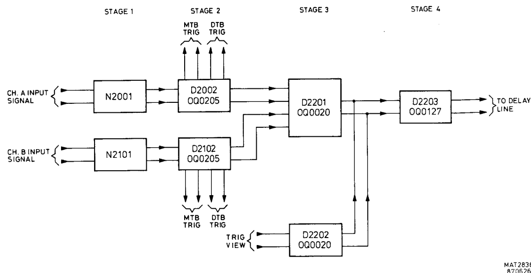
Figure 5.1 The four stages of the vertical pre-amplifier
