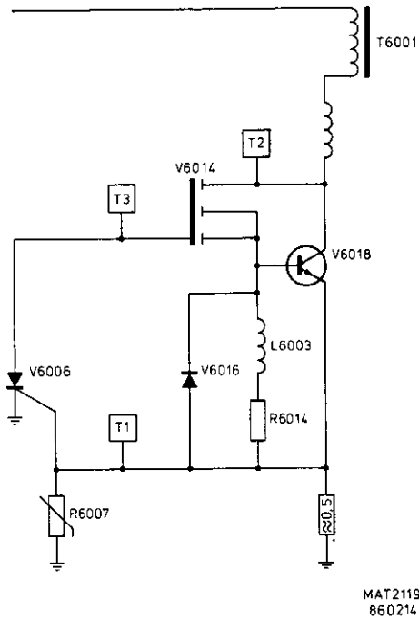
Figure 9.1 Converter circuit
