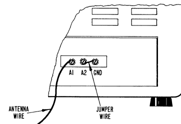
Fig. 4. Single Wire Antenna
