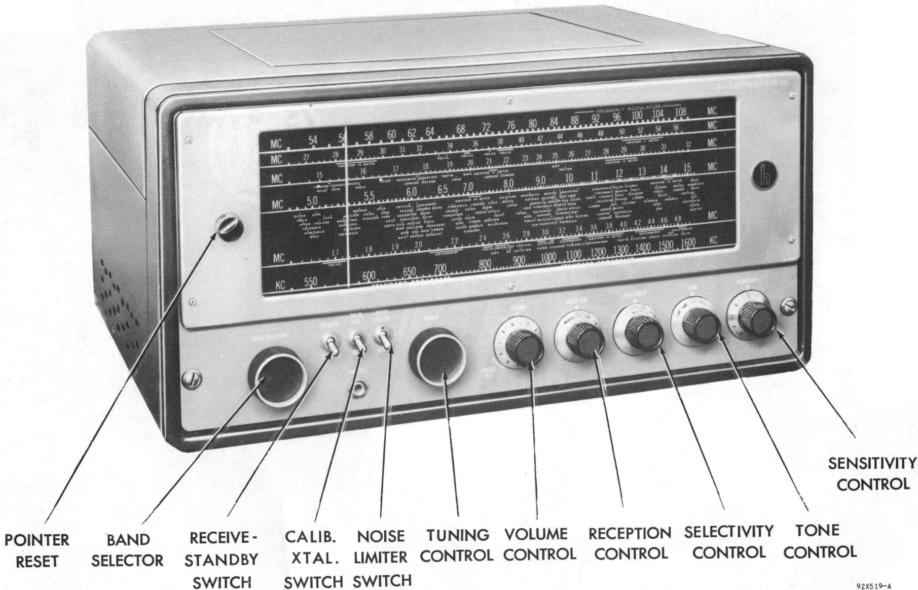
Fig. 1. Radio Receiver Model SX-62A/62AU
