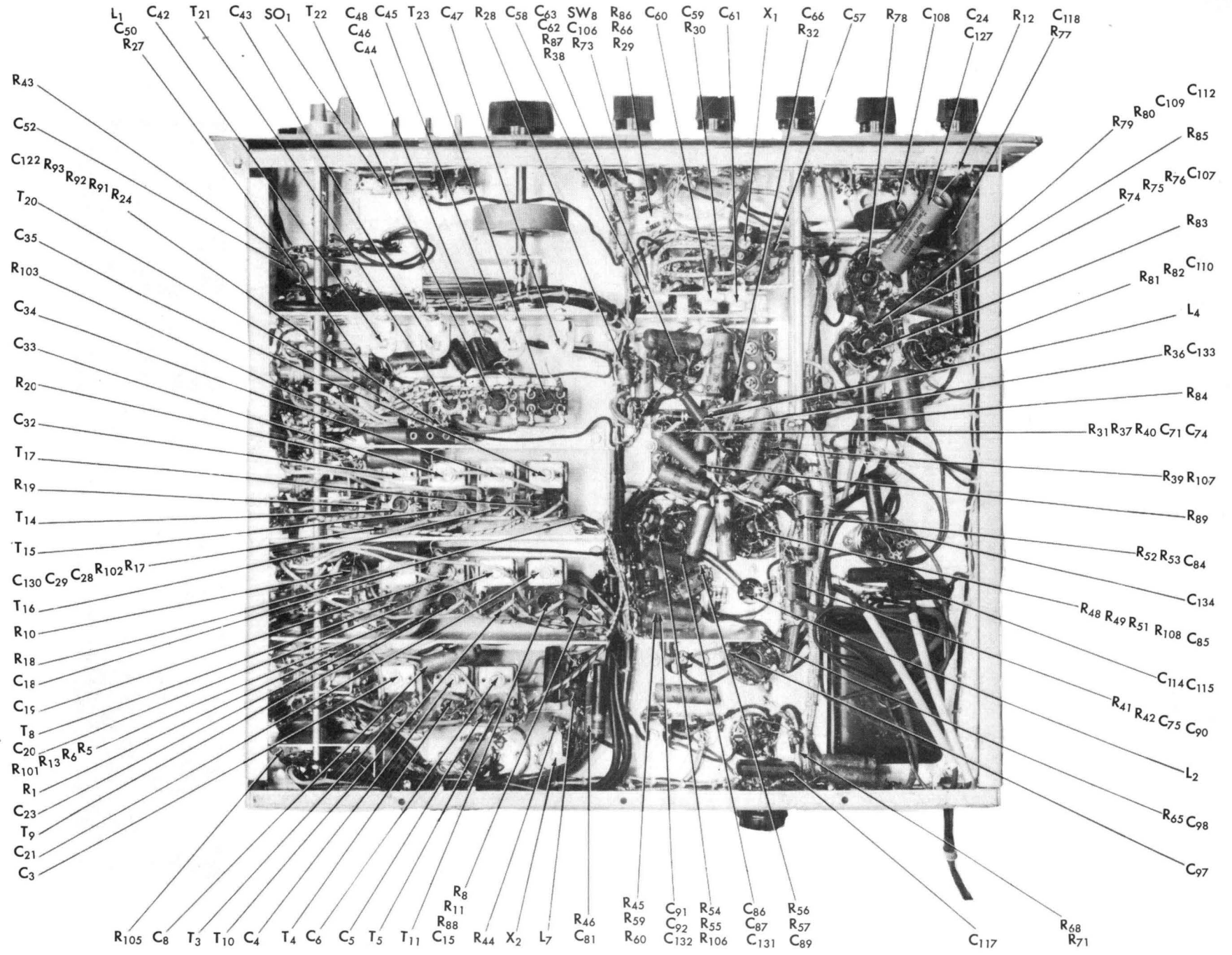
Fig. 13. Component locations, bottom view
