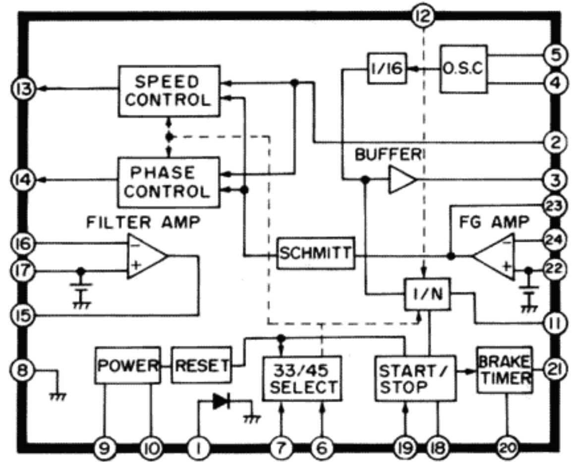
IC201 (AN6680)
