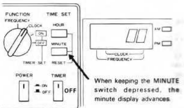
Fig. 3-4 Setting the Time
