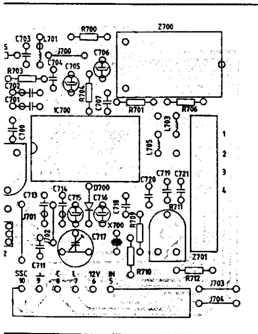
SECAM TRANSCODER
