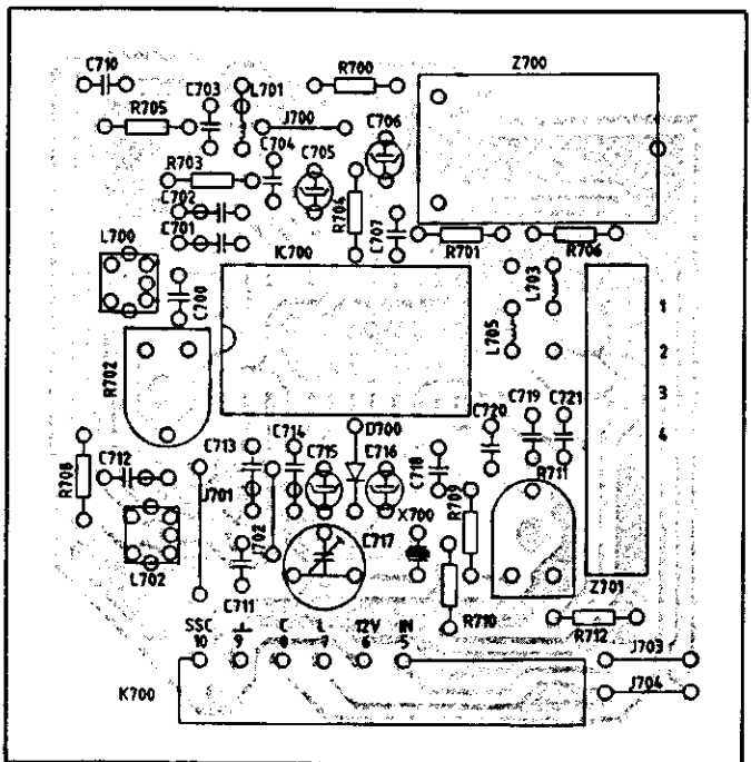
SECAM TRANSCODER
