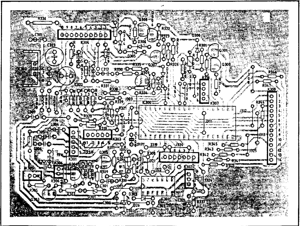
REMOTE BOARD
