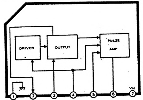
IC701 [AN5515]
