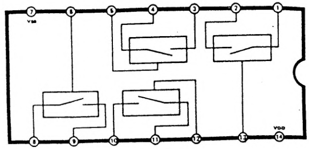
IC351 [TC4066BP]
