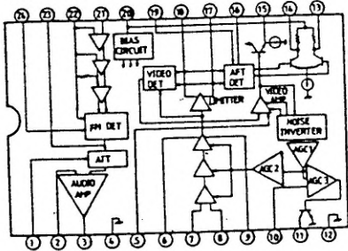
IC251 [TA7680AP]
