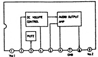
IC851 [ANS265]
