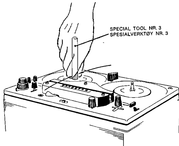
Fig. 4.14 Adjustment of horizontal position.
