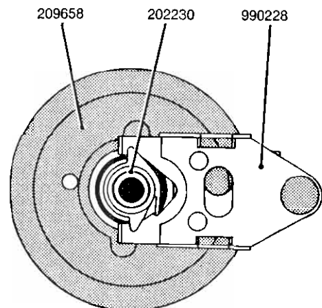
Fig. 4.7 Friction disc with clutch lever.
