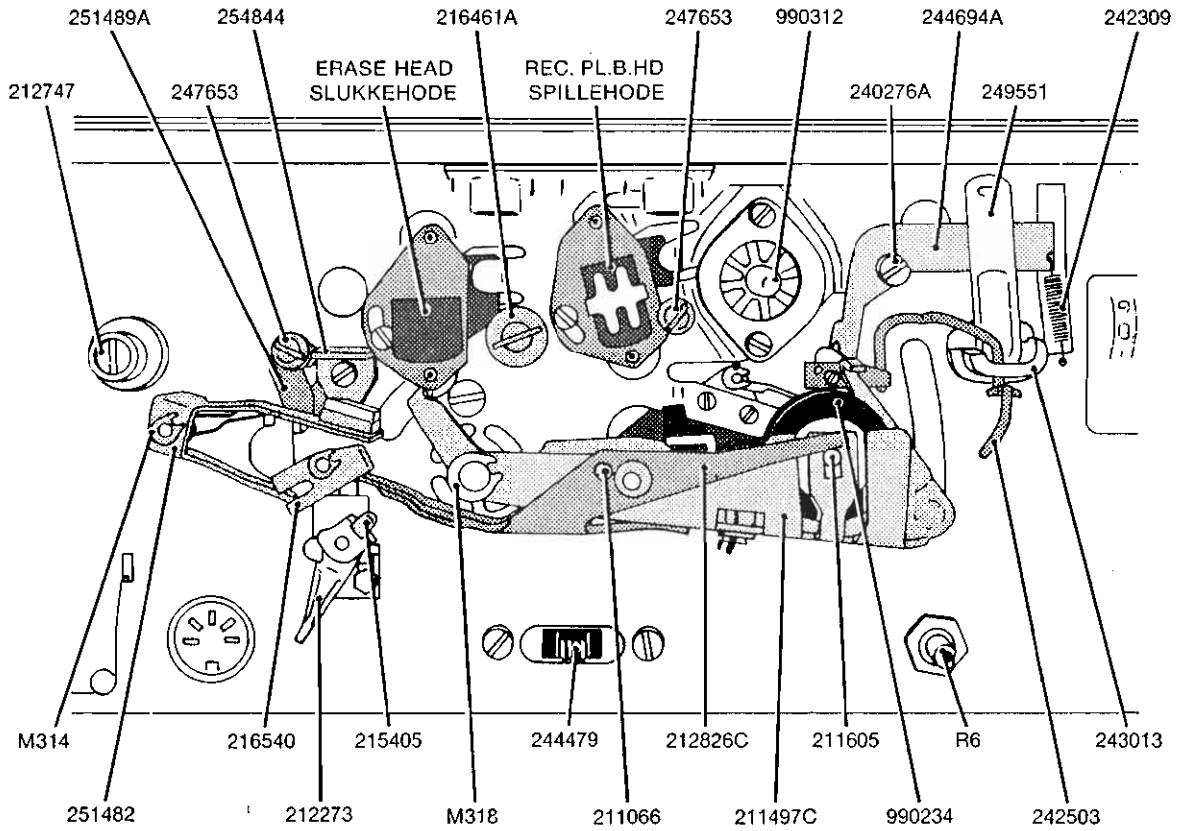
Fig. 4.4 Tape path.
