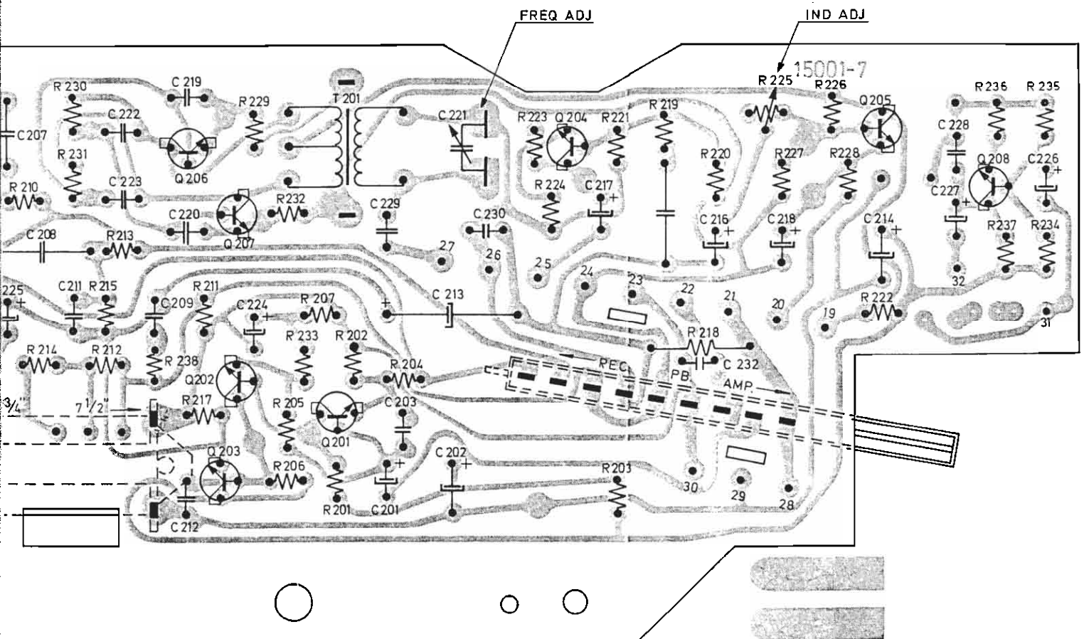
Power amplifier and oscillator, all models. Seen from print side.
