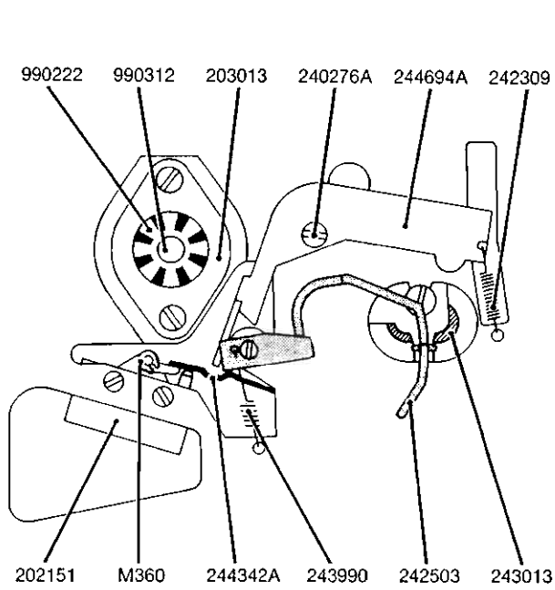
Fig. 4.36 Normal forward drive, winding.
