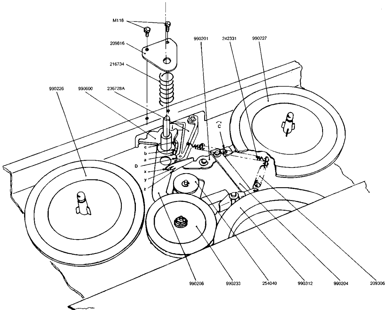
Fig. 4.26 Speed selector mechanism.
