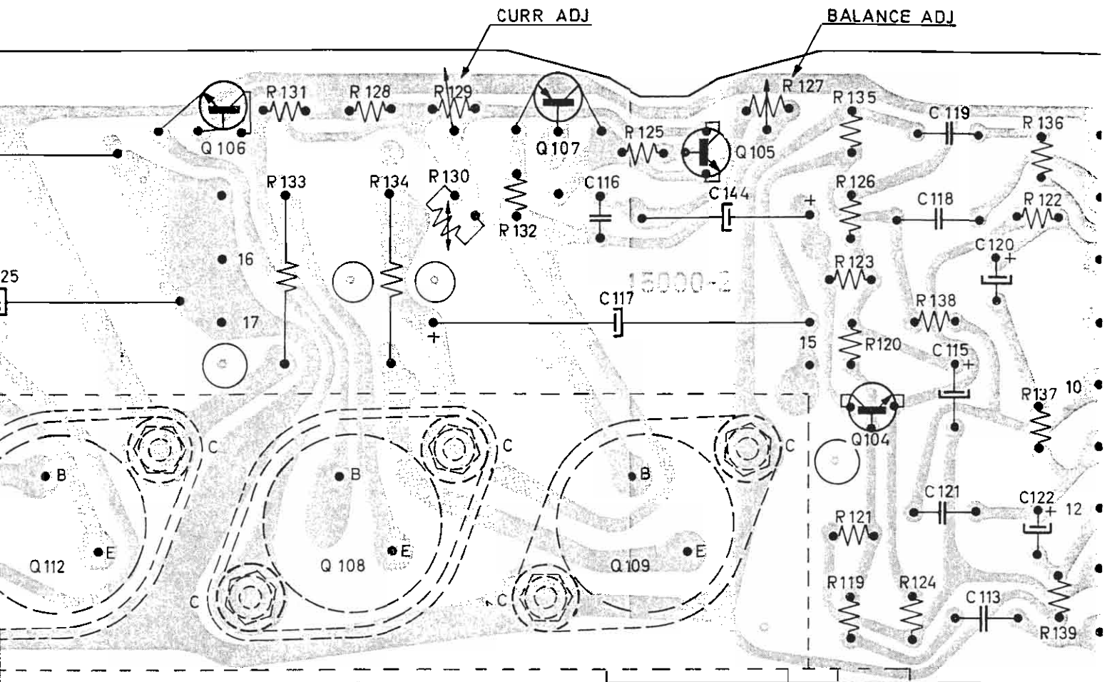
Pre-amplifier and voltage regulator, all models. Seen from print side.
