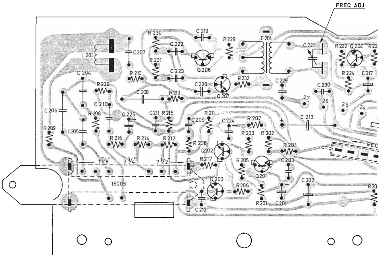
Board for record/playback amplifier, indicator amplifier and oscillator, all models. Seen from print side.
