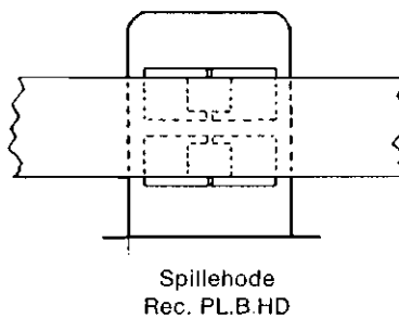
Fig. 6.3 Record/playb. head 2-track model.
