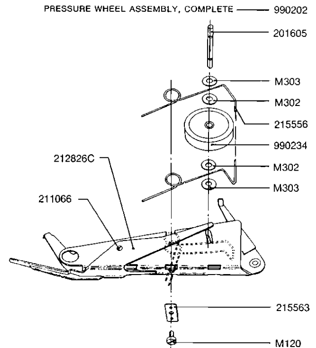
Fig. 4.3 Pressure wheel arm, exploded view.
