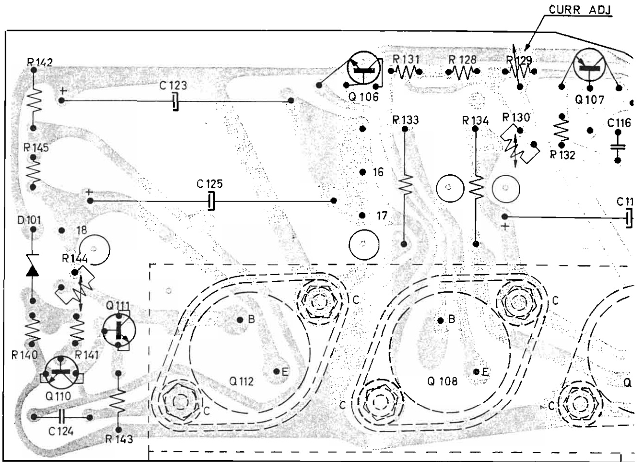
Board for line amplifier, microphone amplifier and voltage regulator, all models. Seen from print side.
