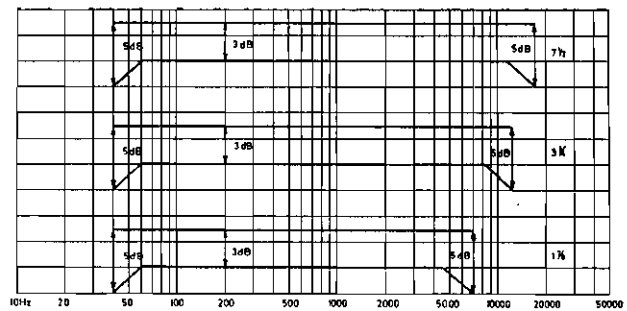
Fig. 8.3 DIN-curves for frequency range.
