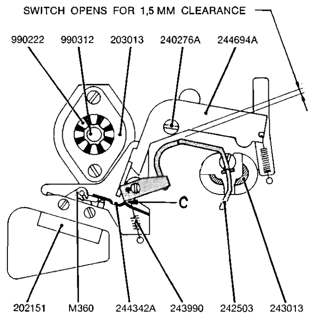
Fig. 4.37 End stop or tape break.
