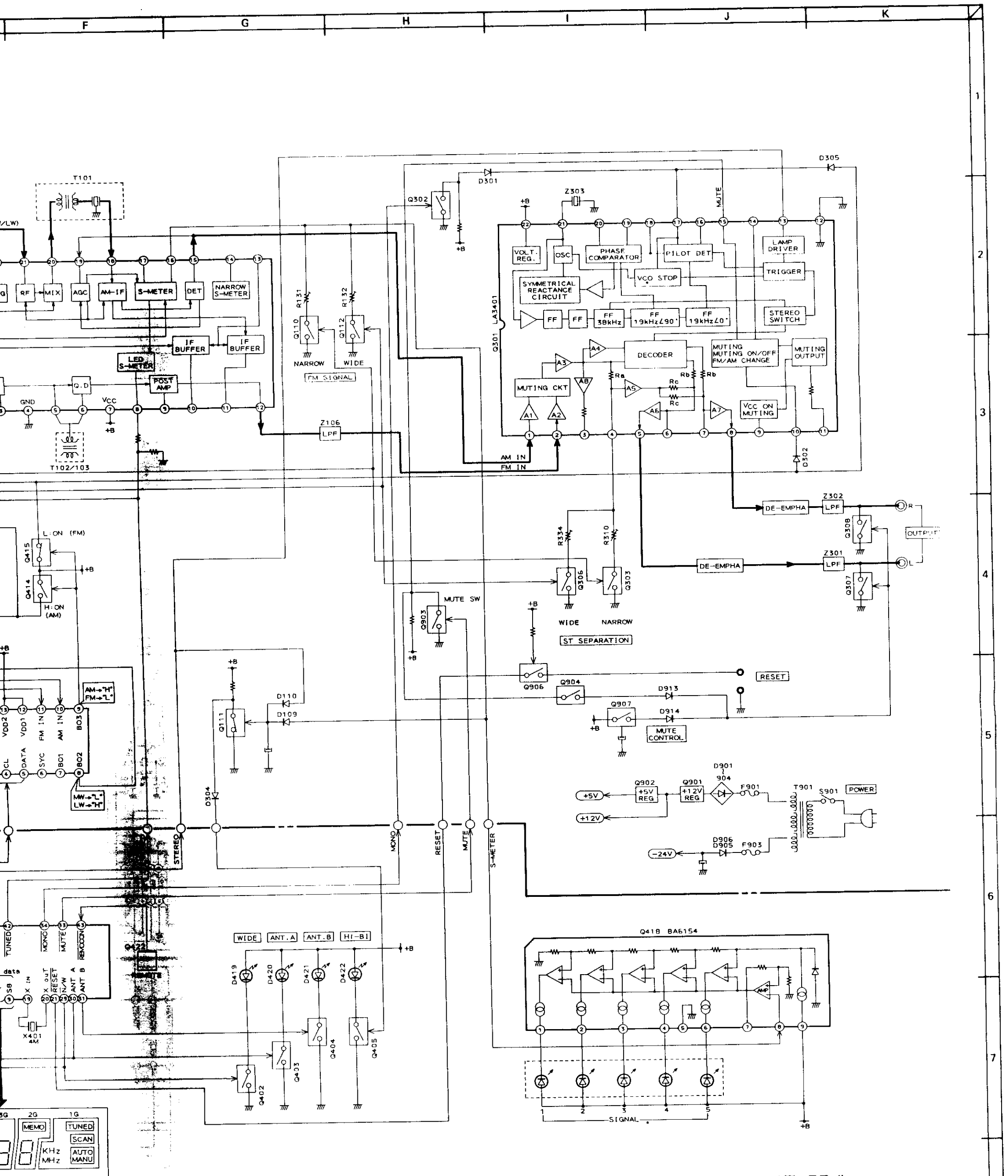
AT-57/L BLOCK DIAGRAM No. A0005 A1
