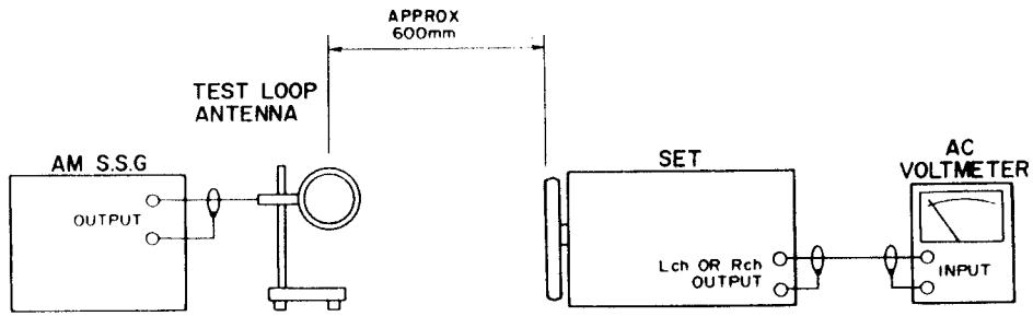
Fig.3-1 Instrument Connection for AM (MW,LW) Section Adjustment
