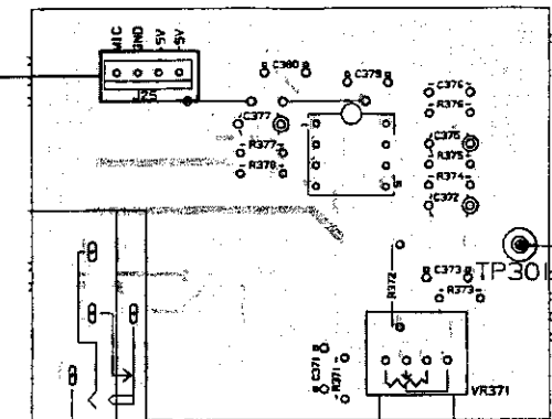
MIC assembly
