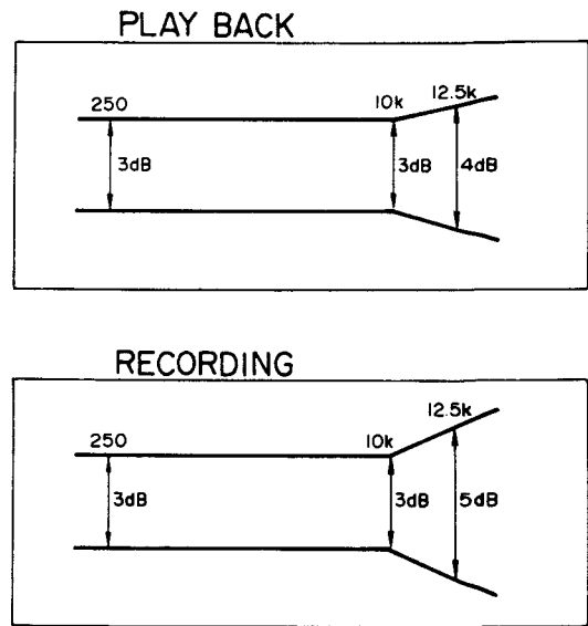
Fig. 6.5 Frequency characteristics
