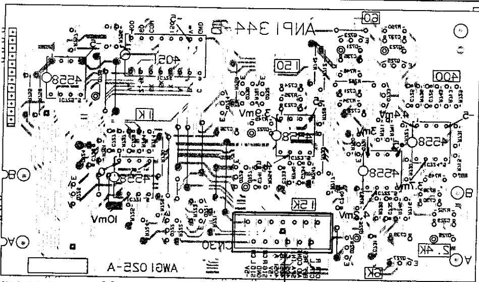
SPANA assembly (AWG1052)
