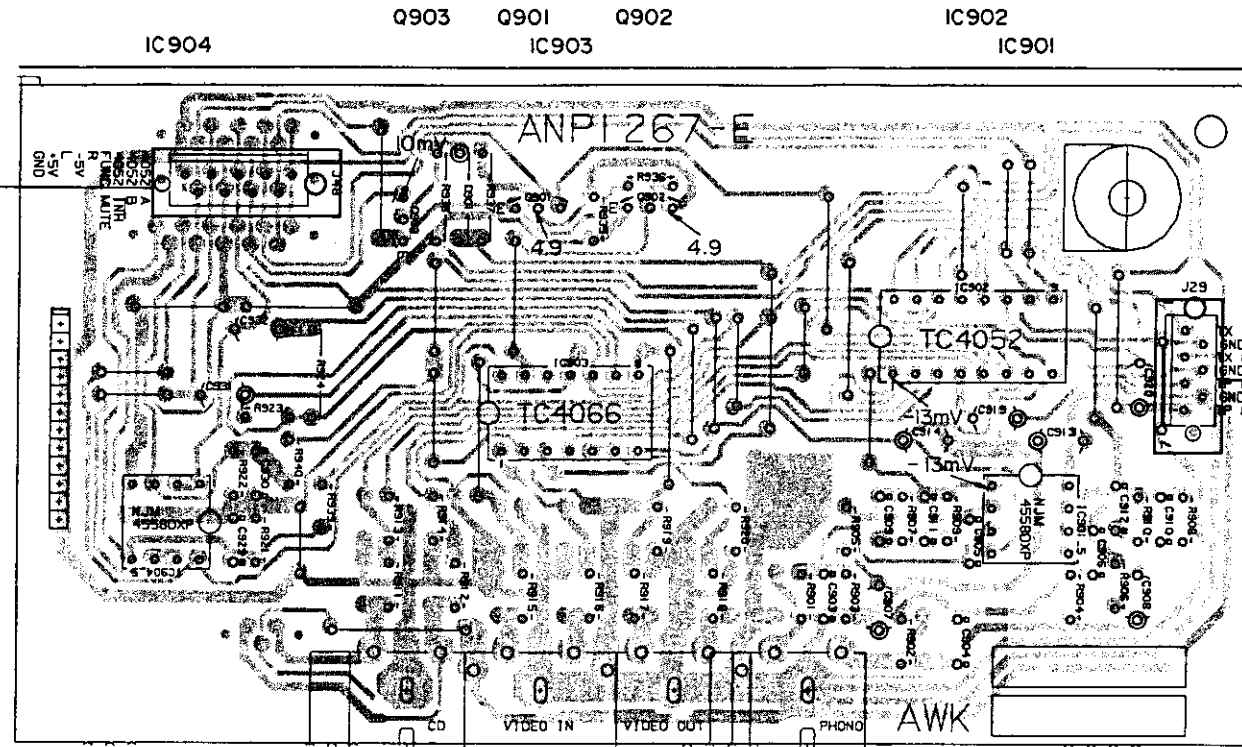
FUNCTION assembly (AWK1174)
