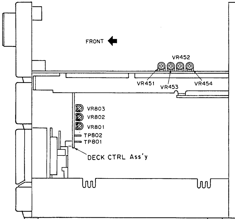
Fig 6.2. Adjustment location
