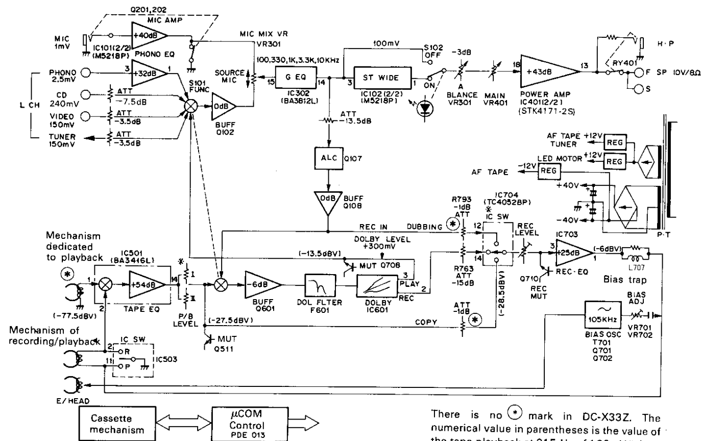
Fig. 10-2-1 Block diagram
