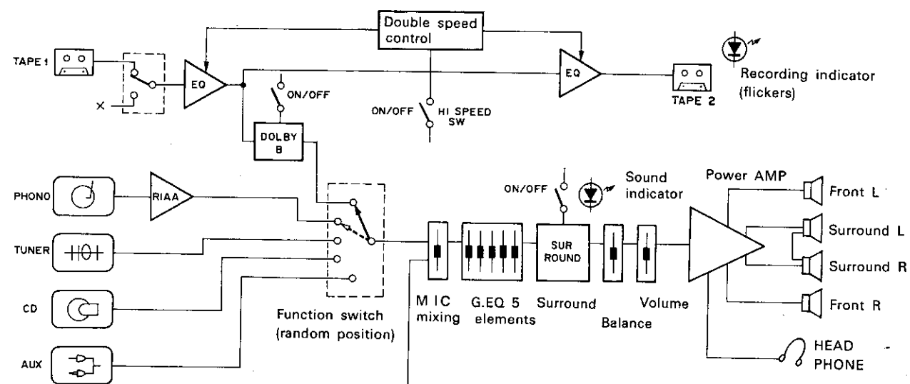
Fig. 10-1-3 Signal system basic block during recording Function TAPE (dubbing) (DC-X55Z only)
