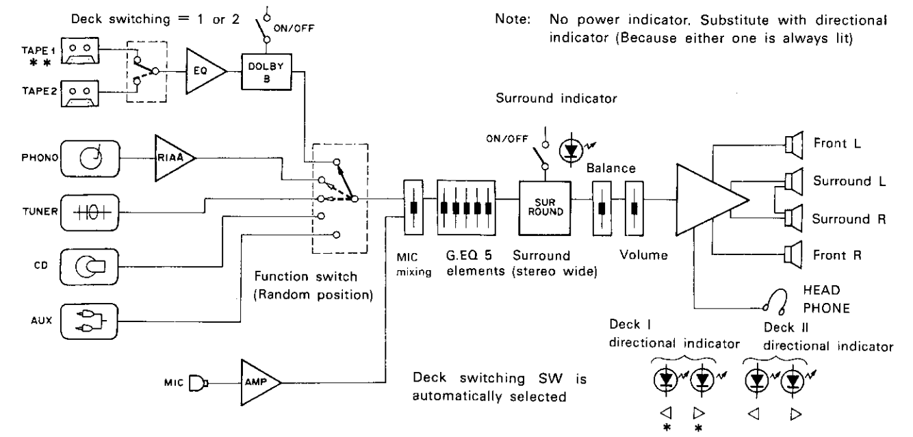
Fig. 10-1-1 Signal system basic block during playback (DC-X55Z, DC-X33Z)
