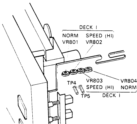
Fig. 12-1 Adjustment Point
