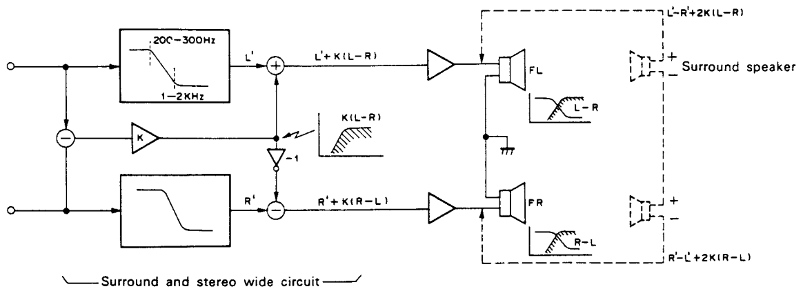
Fig. 10-4-1 Surround and stereo wide circuit block diagram
