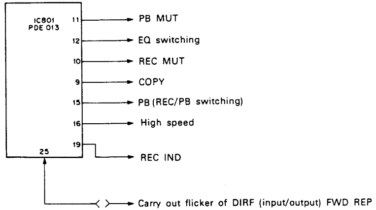
Fig. 10-5-2 Control of microcomputer circuit block dedicated to control
