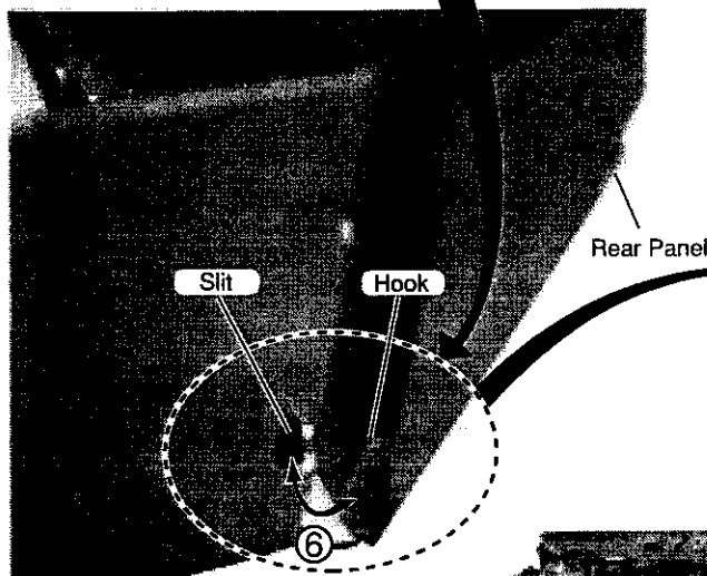
The Hook of a rear panel is put in to a slit.
