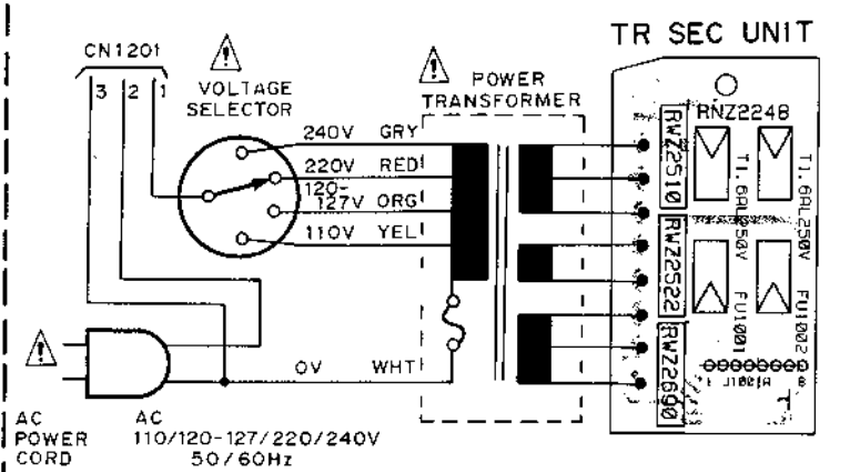
Power Supply Section for HEM and HB Types.
