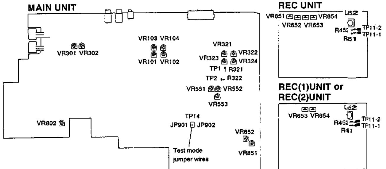
Fig. 8-2 Adjusting points
