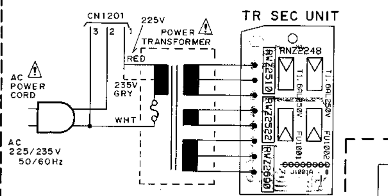
Power Supply Section for HEM and HB Types.
