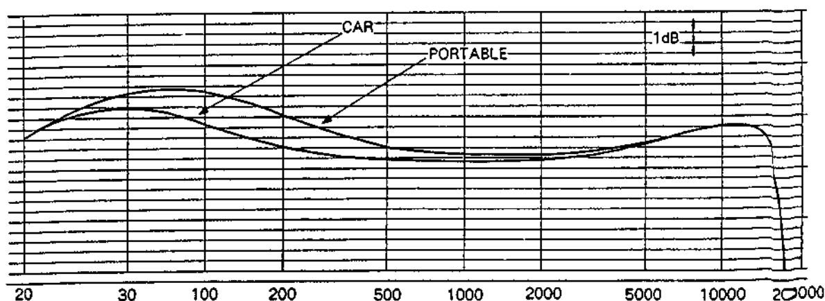
FREQUENCY RESPONSE (LINE) MPX ON
