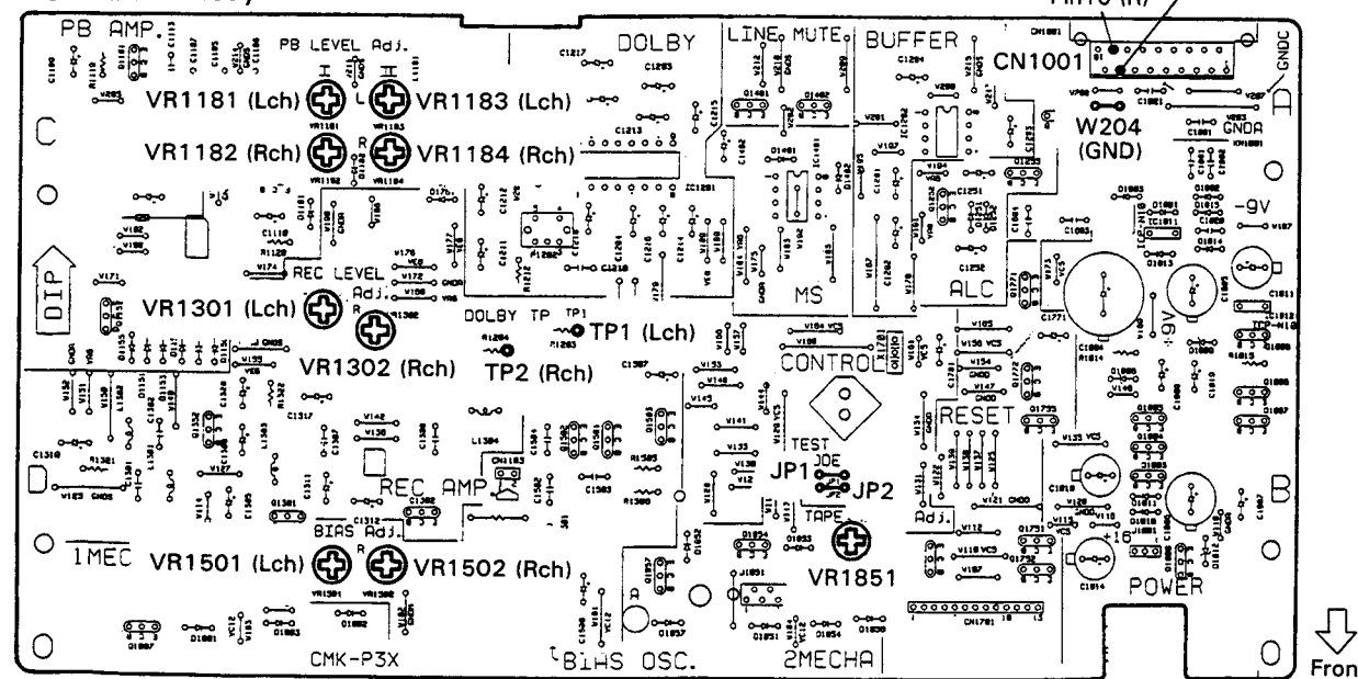
Fig. 2-4 Adjustment and Measurement Points
