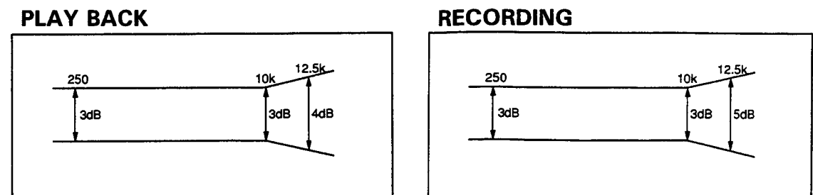
Fig. 2-2 Frequency Characteristics
