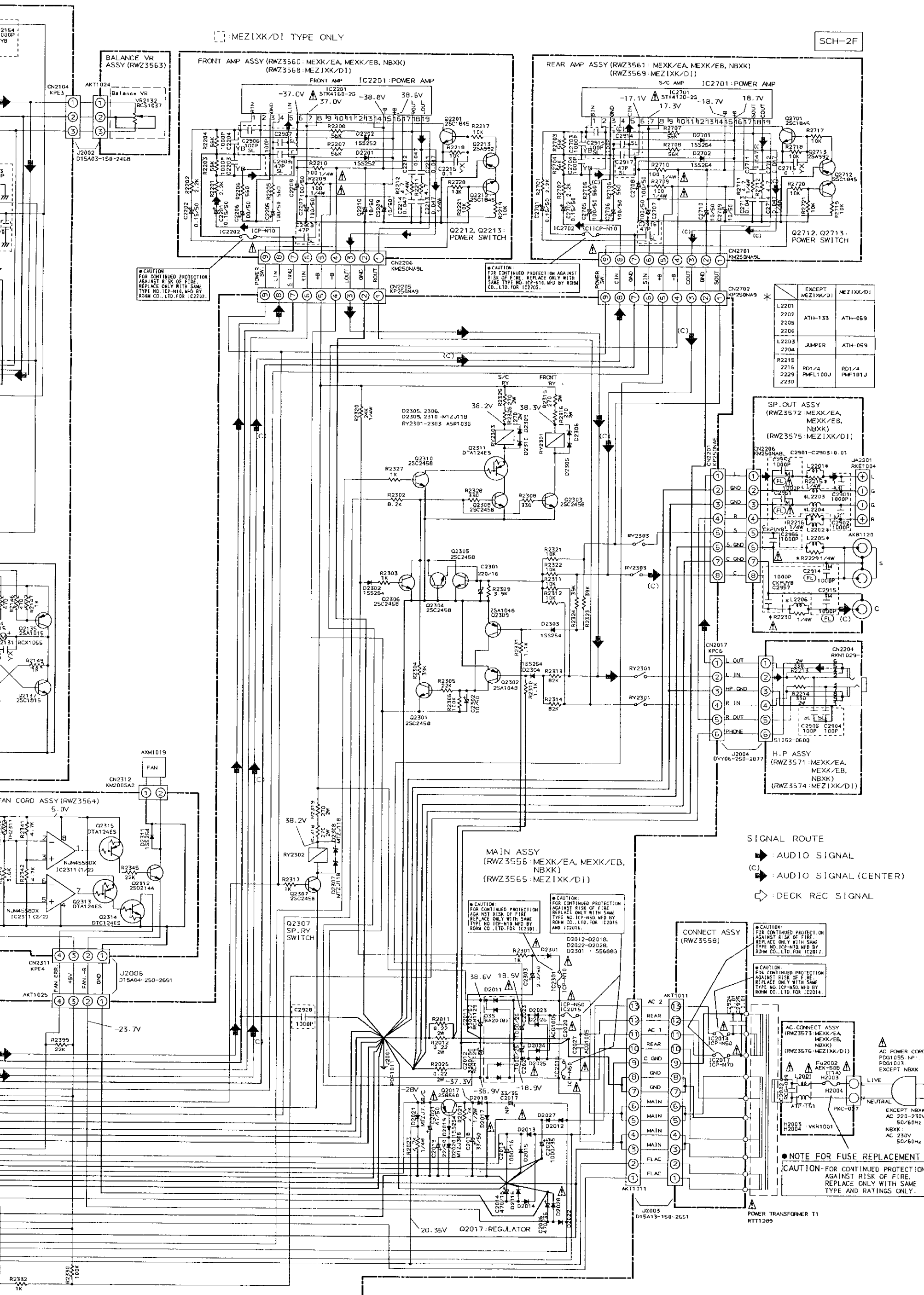
MAIN ASSY, SFC. VR ASSY, CONNECT ASSY, PRO. LOGIC ASSY, FRONT AMP ASSY, REAR AMP ASSY, REGULATOR ASSY, BALANCE VR ASSY, FAN CORD ASSY, H. P. ASSY, SP. OUT ASSY, AC. CONNECT ASSY
