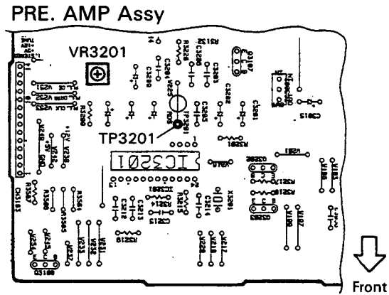
Fig. 1-4 Adjustment Points
