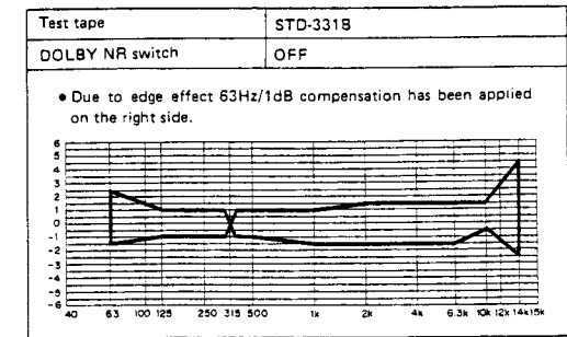
Fig. 9-3 . Allowable playback frequency response zone
