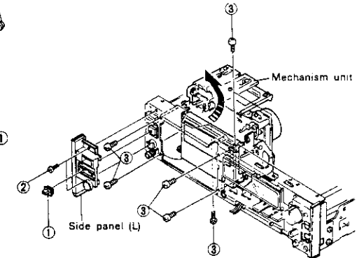
Fig. 3-3. Removal of mechanism unit
