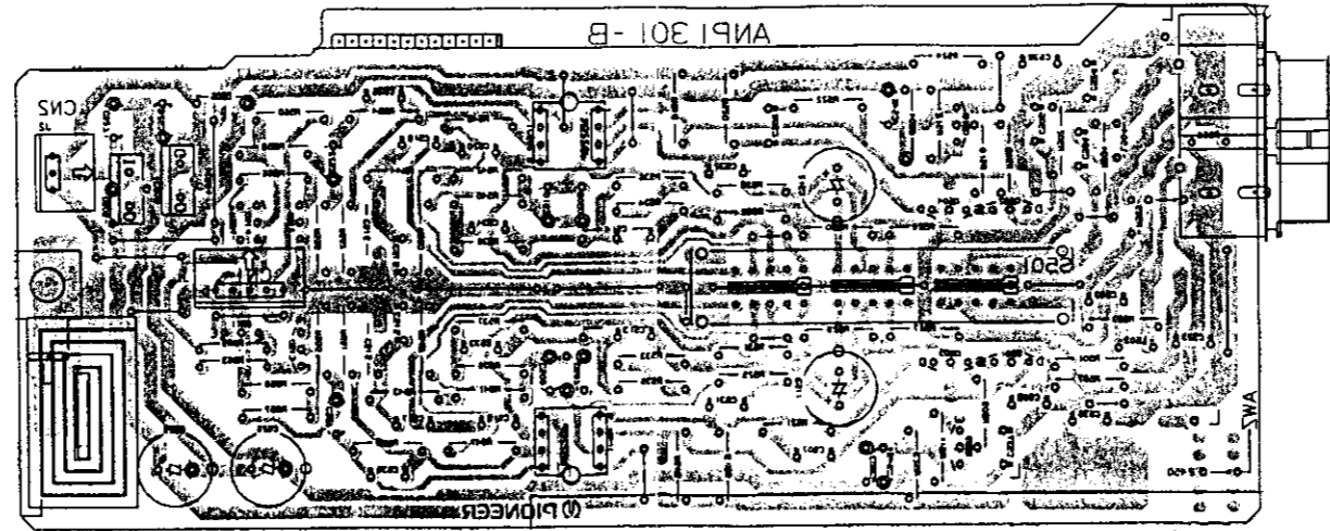
PHONO AMP assembly (W22450)
