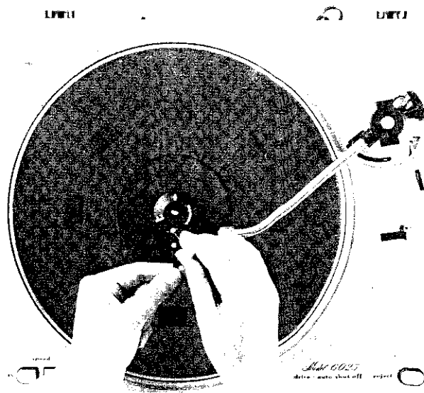
Figure 2 Stylus Overhang Adjustment
