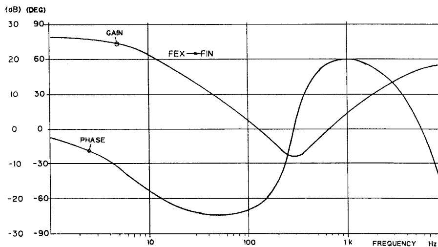
Fig.15 : FOCUS EQUALIZER
