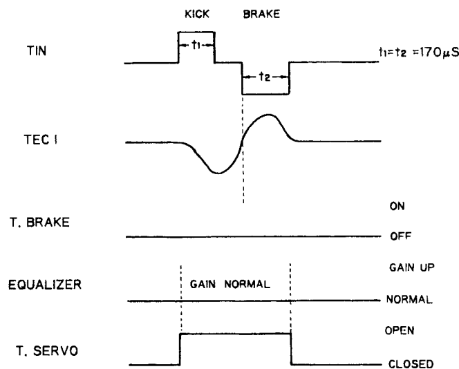
Fig.21 : SINGLE TRACK JUMP
