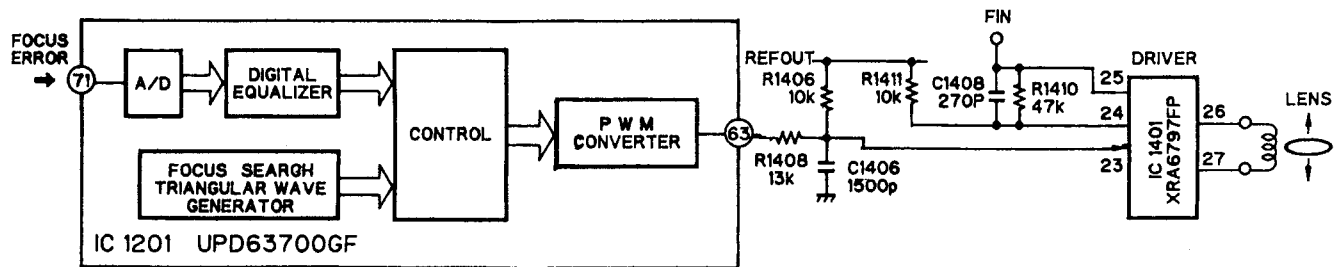
Fig.14 : FOCUS SERVO BLOCK DIAGRAM
