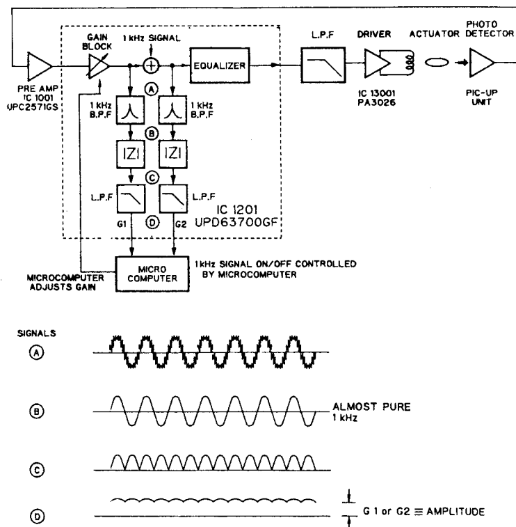
Fig.29 : AGC BLOCK DIAGRAM
