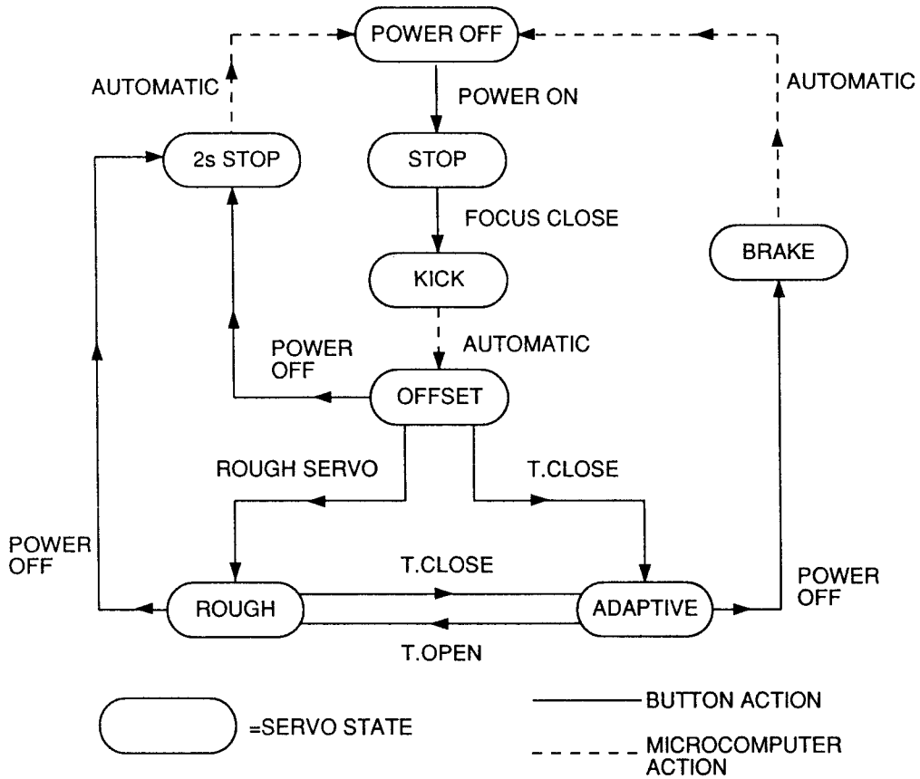
Fig.28 : SPINDLE SERVO MODES
