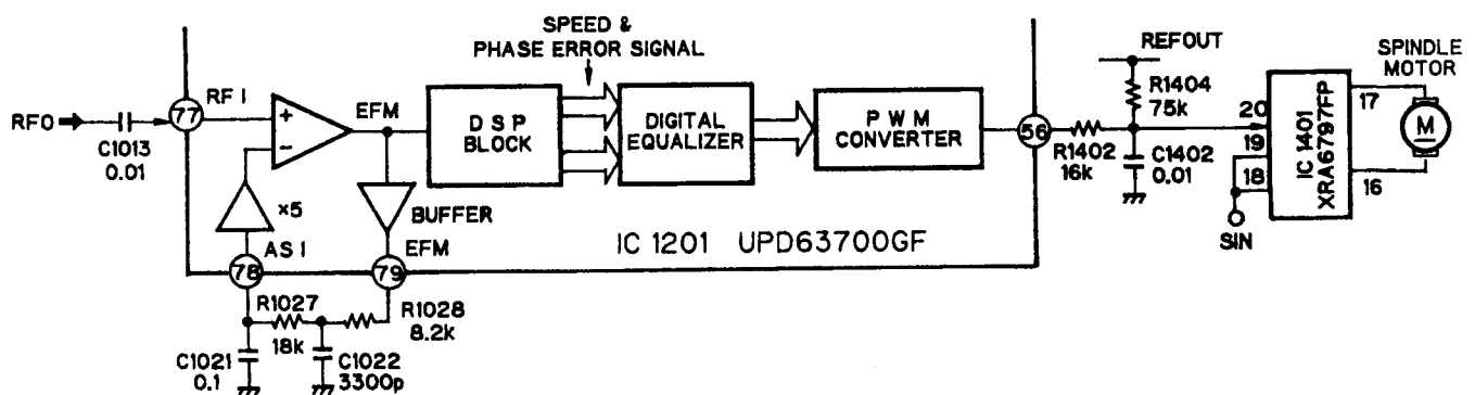
(EFM Compalator Circuit)
