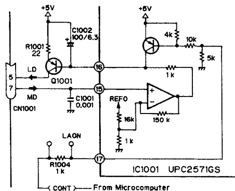
Fig.9 : APC CIRCUIT
