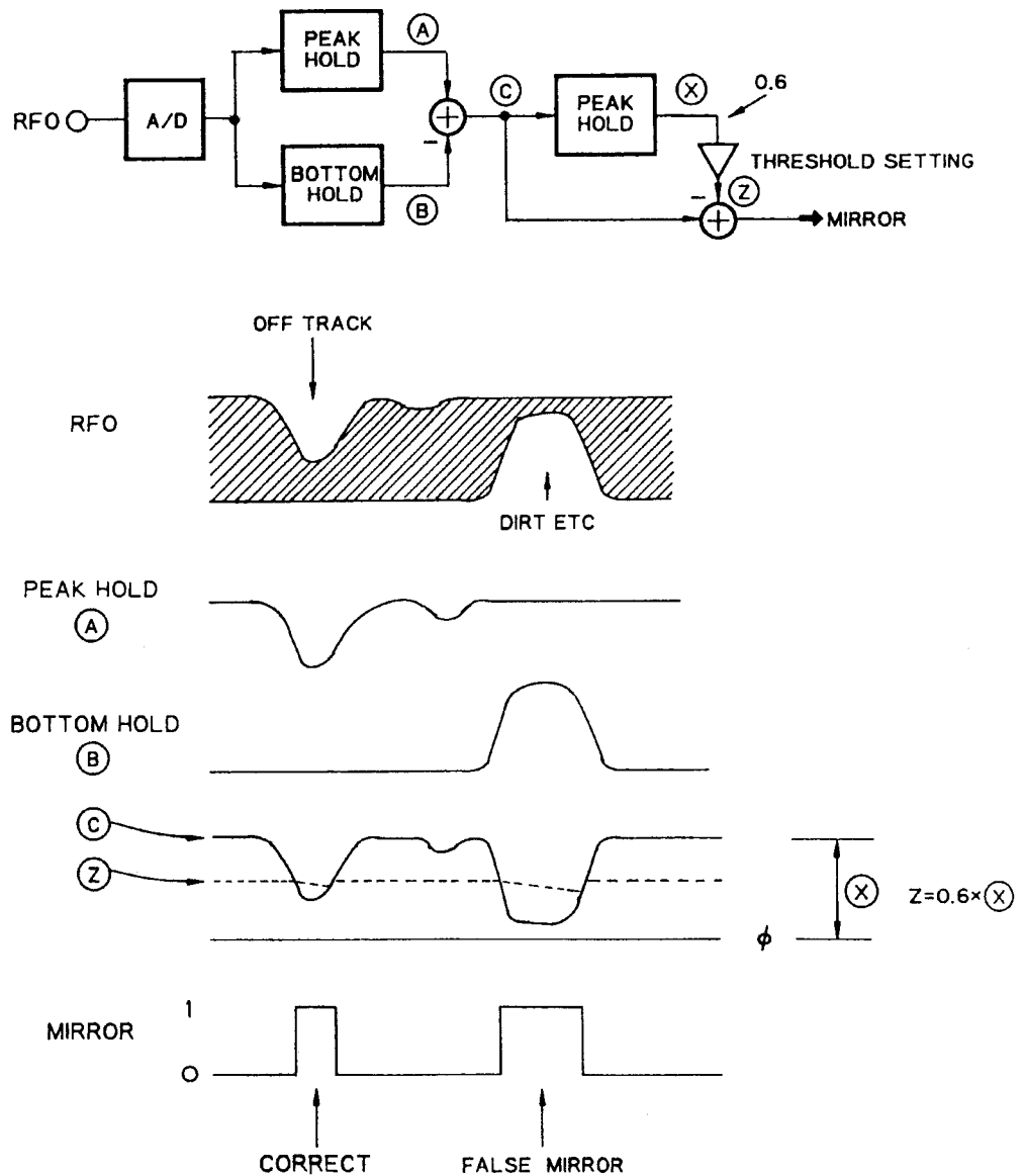
Fig.24 : MIRROR CIRCUIT & SIGNAL DIAGRAM
