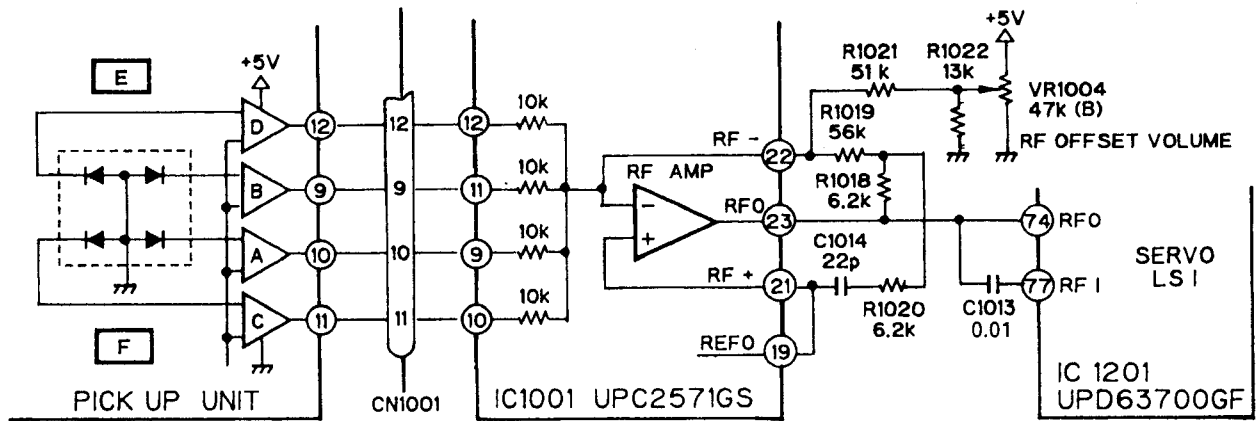
Fig.10 : RFO AMPLIFIER
