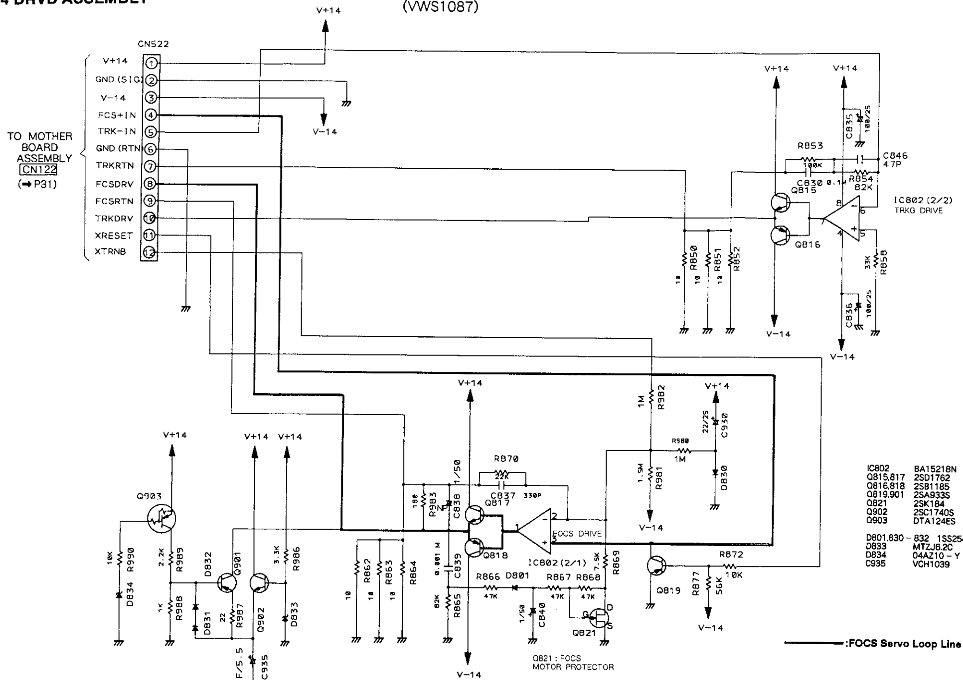
DRVB ASSEMBLY
