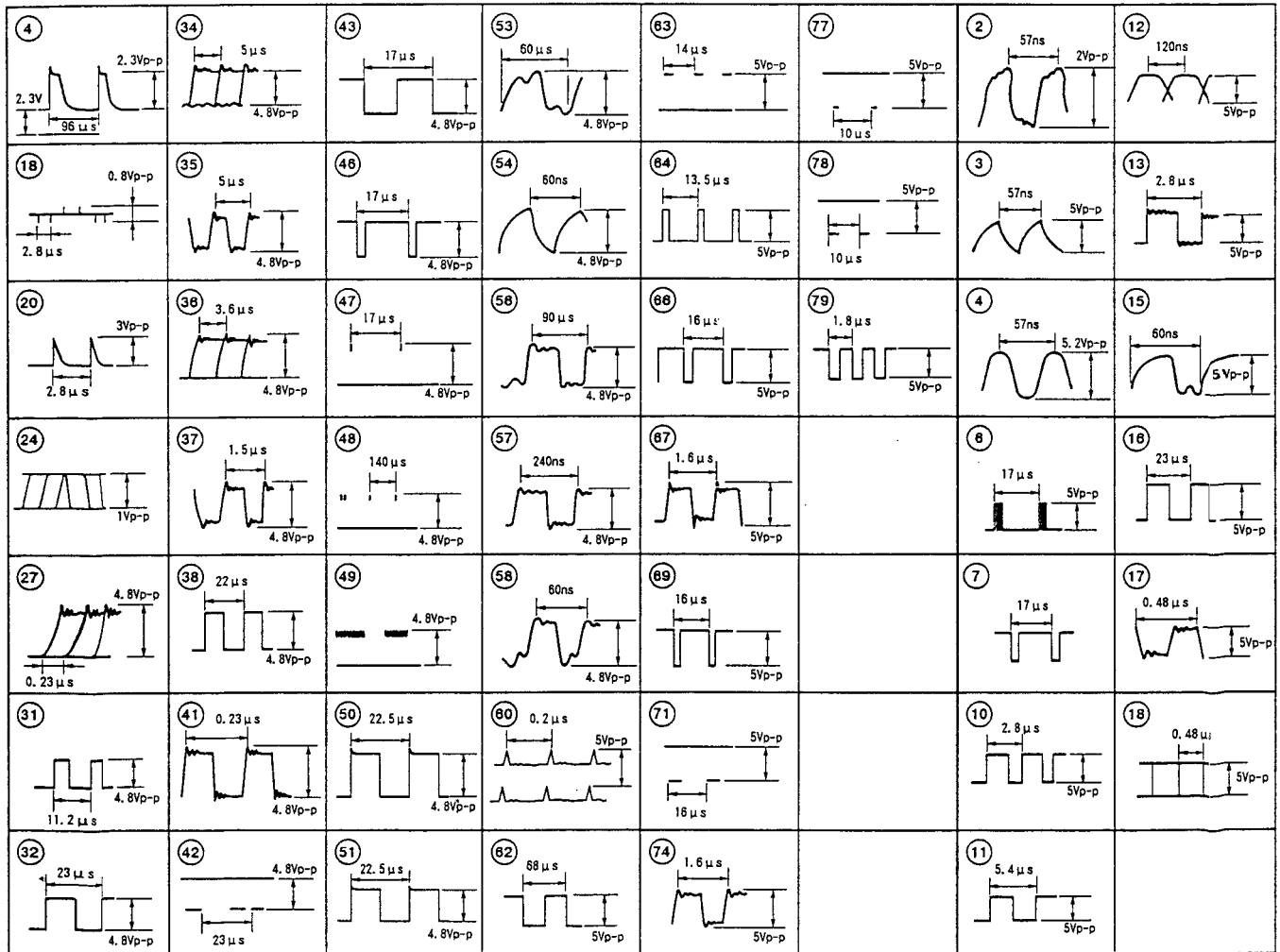
IC201 (CXD2500AQ)
