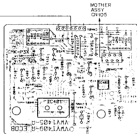
ECOB ASSY
