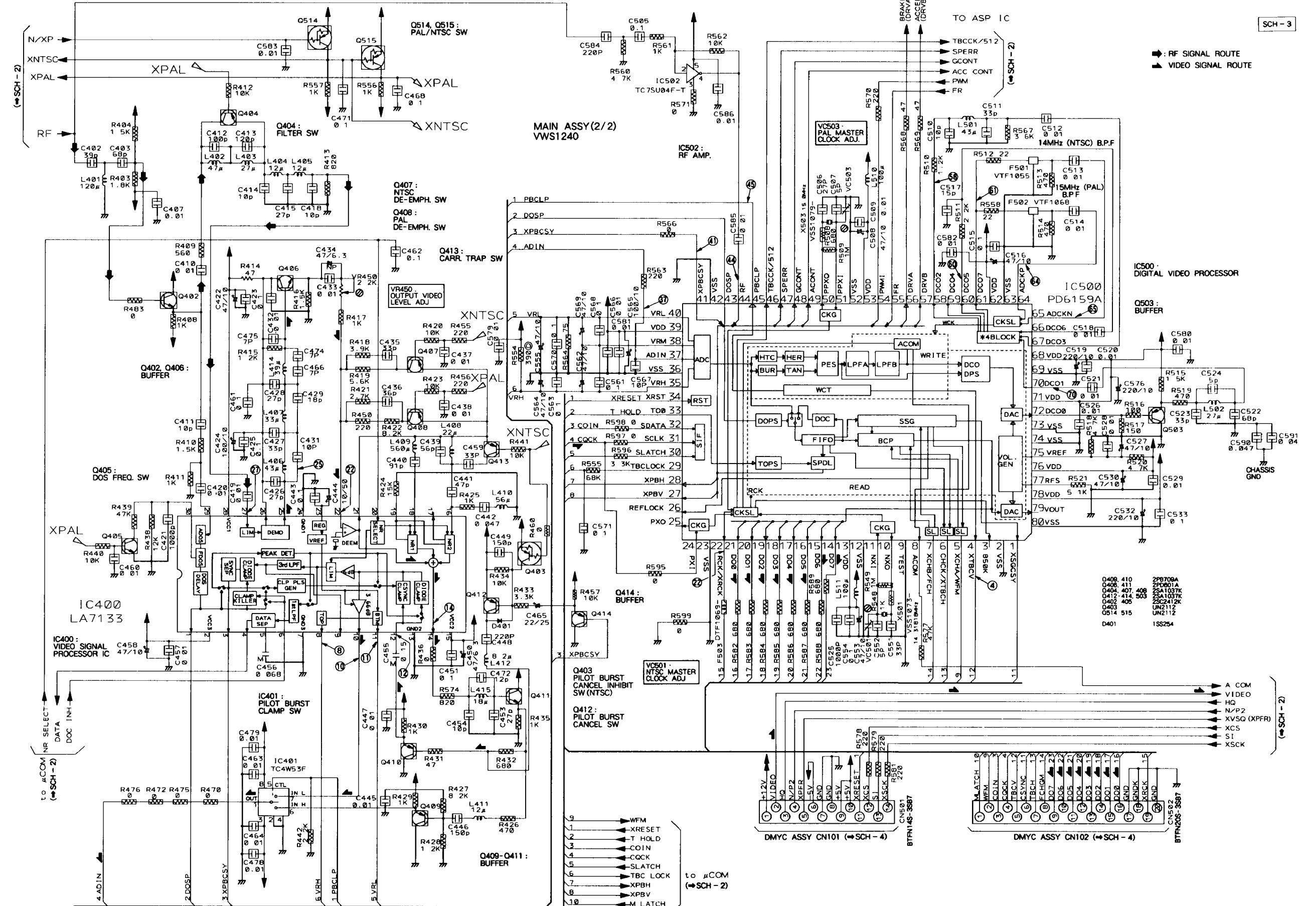
SCH-3 MAIN ASSY (2/2)
