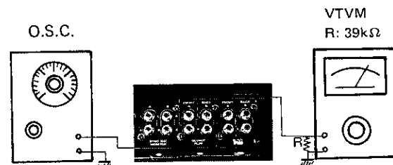
RTU-11 Rear panel
