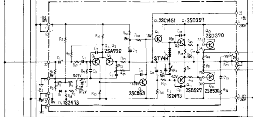
POWER AMP ASSY AWH-027 (B) REAR R Ch
