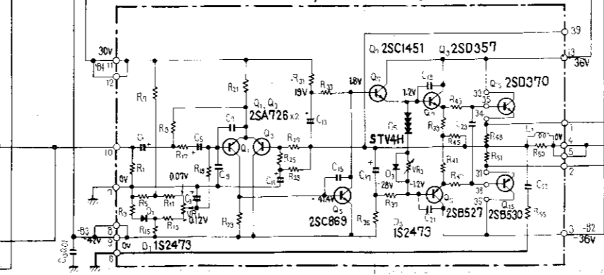
POWER AMP ASSY AWH-027 (A) REAR L Ch
