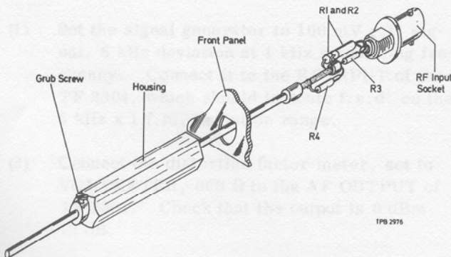
Fig. 5.1 Attenuator assembly
