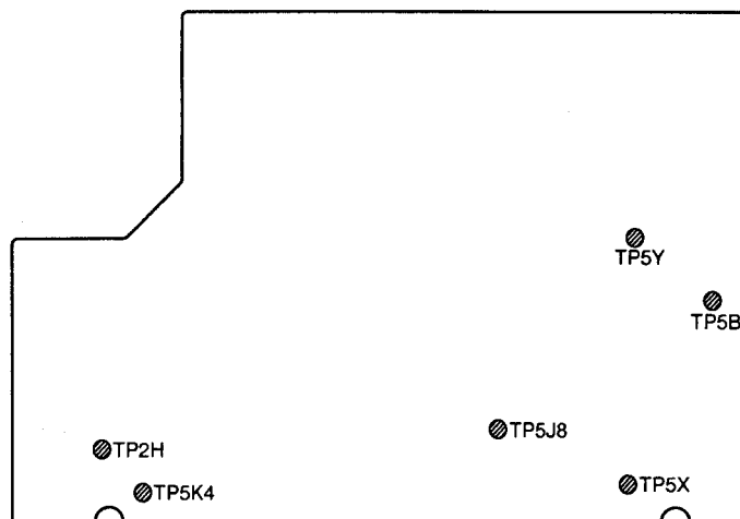
PCB-MAIN(Component side)
