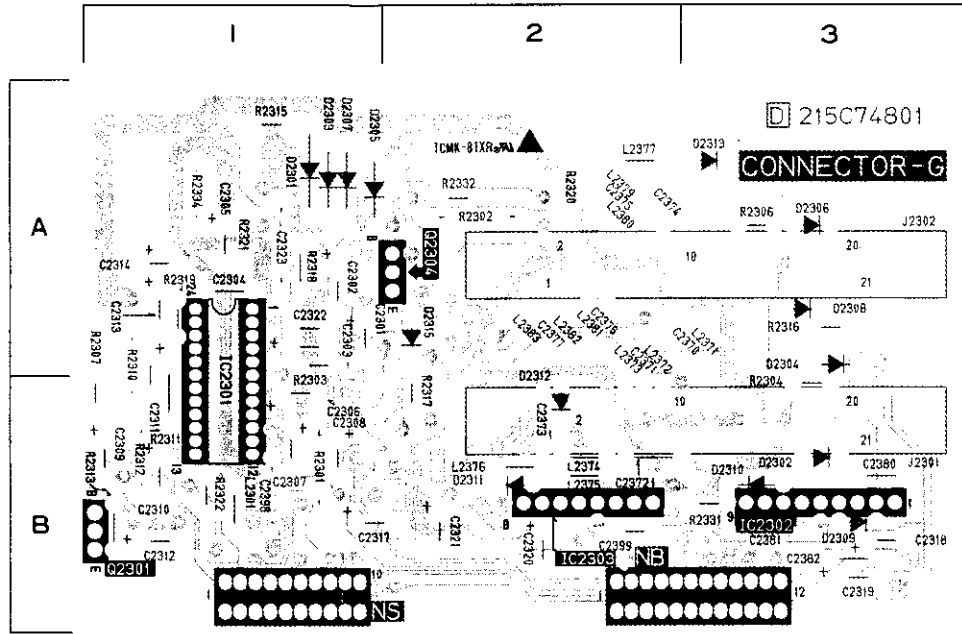
PCB-CONNECTOR-G [SOLDER SIDE] (HS-M20V(G) only)
