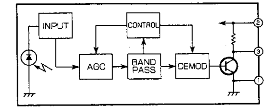
Z8A0 PREAMAP
