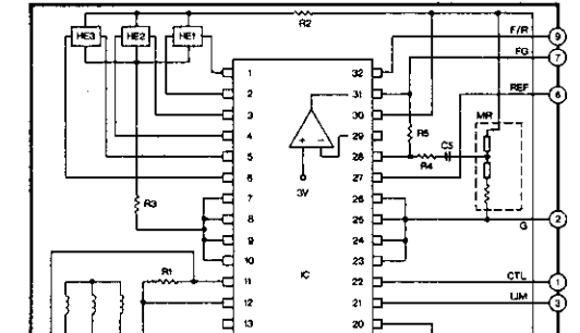
CAPSTAN MOTOR
