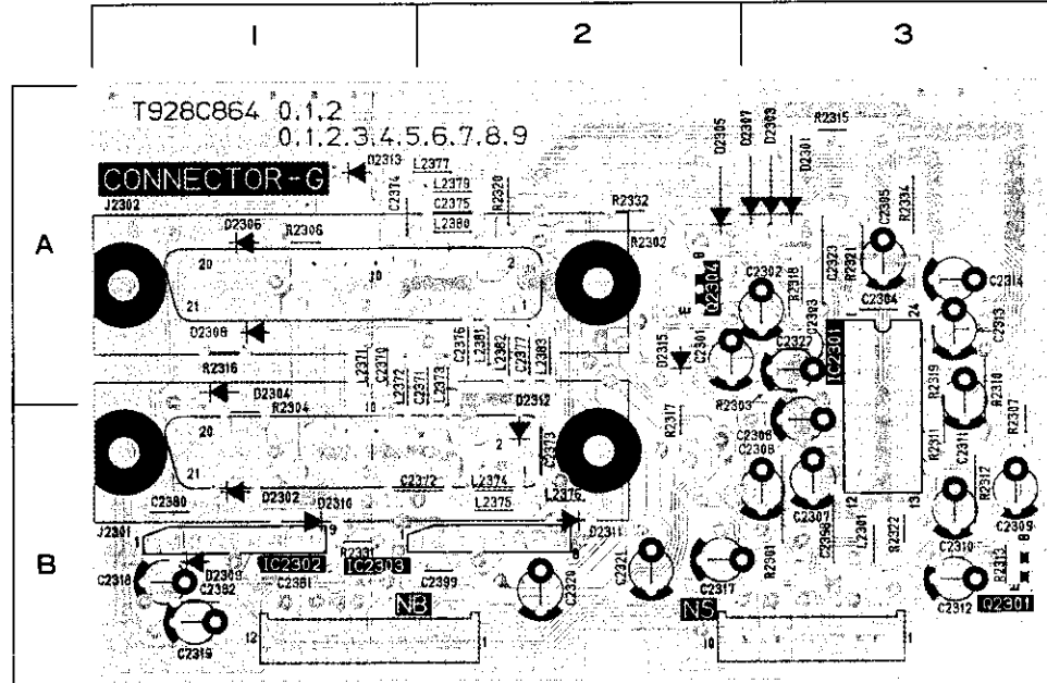
PCB-CONNECTOR-G [COMPONENT SIDE] (HS-M20V(G) only)
