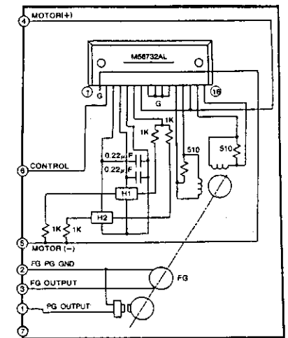
CAPSTAN MOTOR
