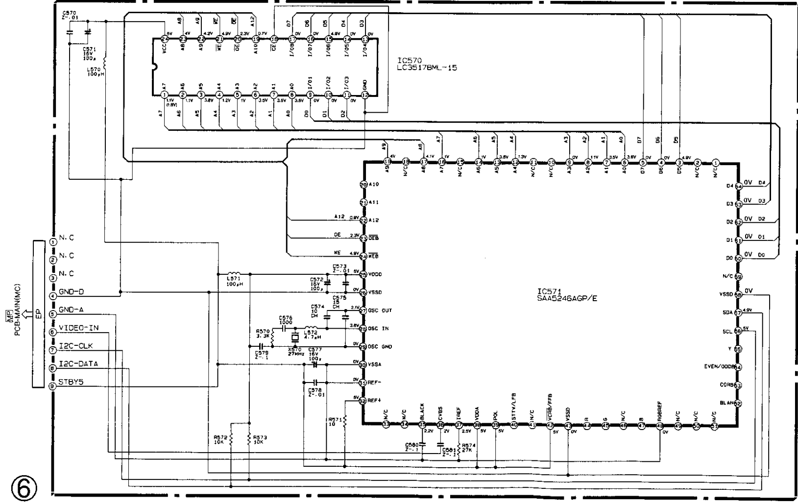
△ PCB-TEXT ONLY FOR HS-M20V(B)
