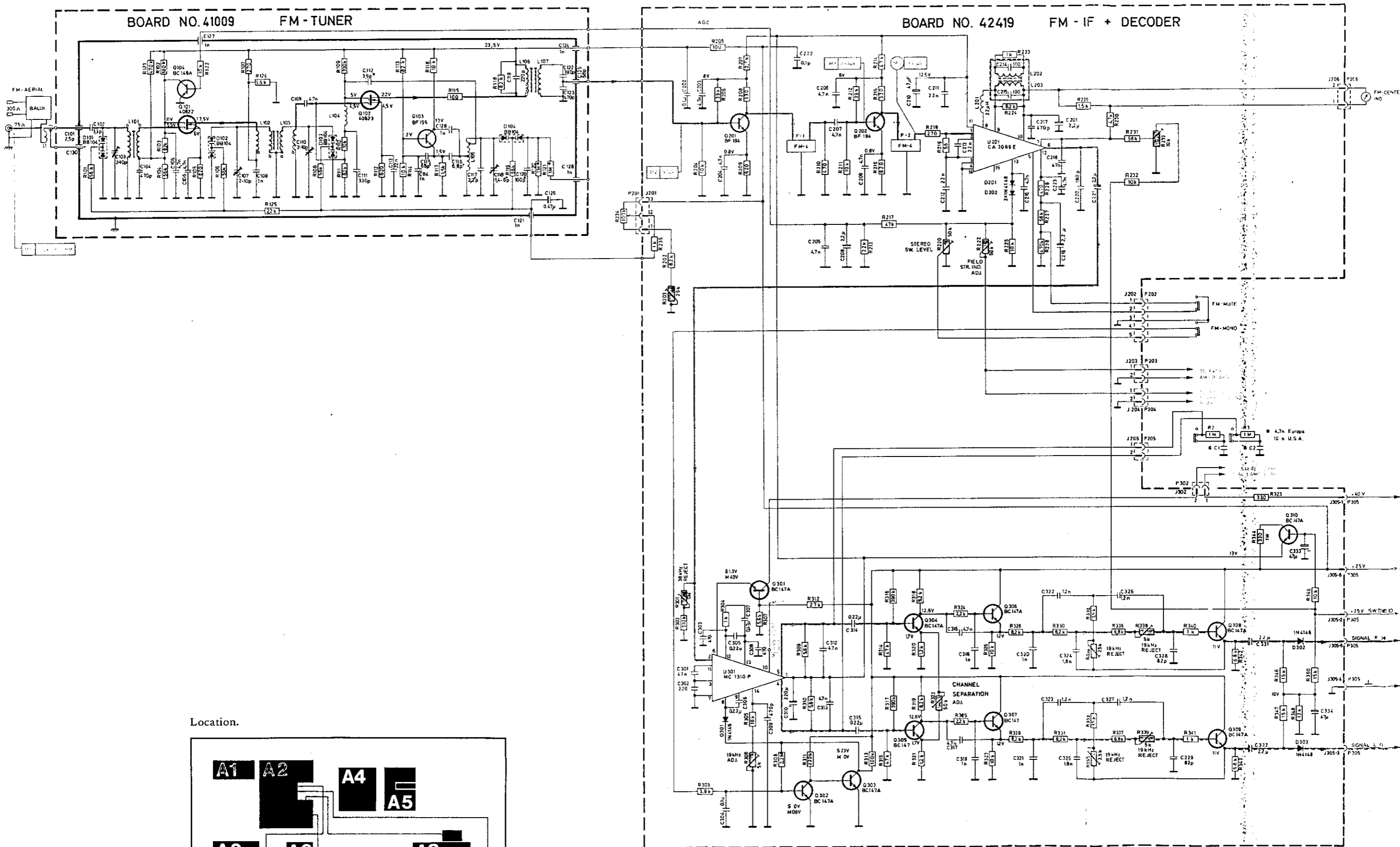
FM-IF SECTION - 42598
