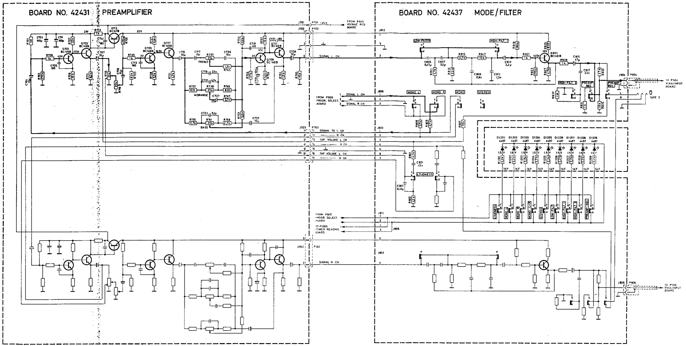
AUDIO SECTION 2 - 43551
